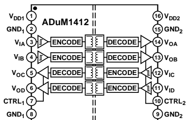
図3.ADuM1412
