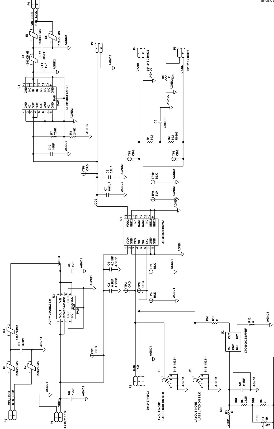
Figure 4. EVAL-ADM3050EEBZ Schematic
