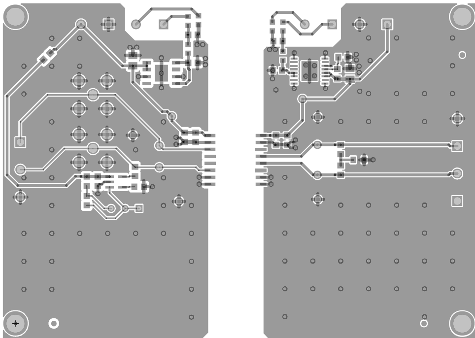
Figure 6. EVAL-ADM3050EEBZ Top Layer
