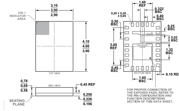
Figure 73. 26-Lead Land Grid Array [LGA] 3 mm × 4 mm (CC-26-2) Dimensions shown in millimeters
