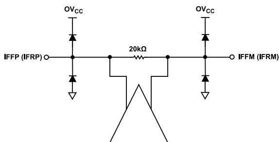
Figure 62. Simplified Schematic of the IF Output Interfaces
