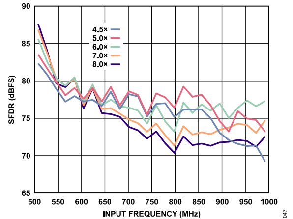
Figure 44. Buffer Current Sweeps (SFDR vs. Input Frequency and I_{BUFF} ), 500 MHz < f_{IN} < 1000 MHz
