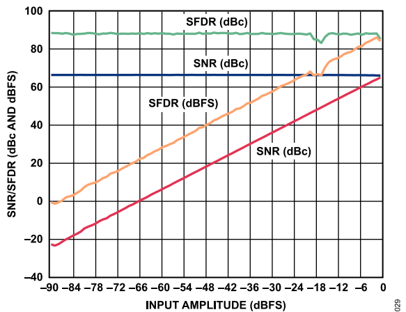
Figure 26. SNR/SFDR vs. Input Amplitude, f_{IN} = 170.3 MHz
