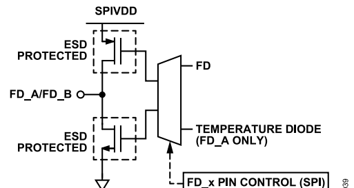
Figure 36. FD_A/FD_B Outputs
