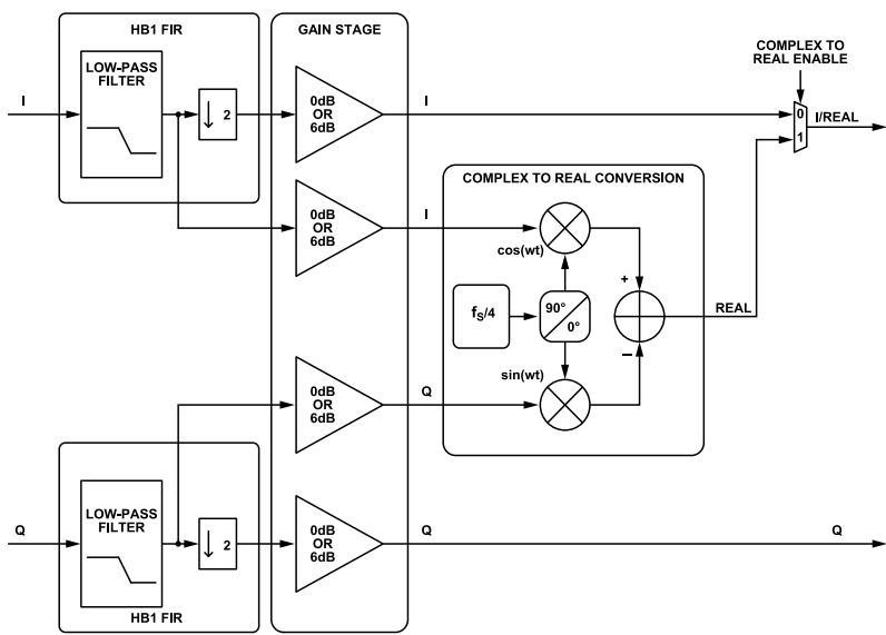
Figure 66. Complex to Real Conversion Block
