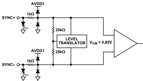
Figure 31. SYNC± Inputs
