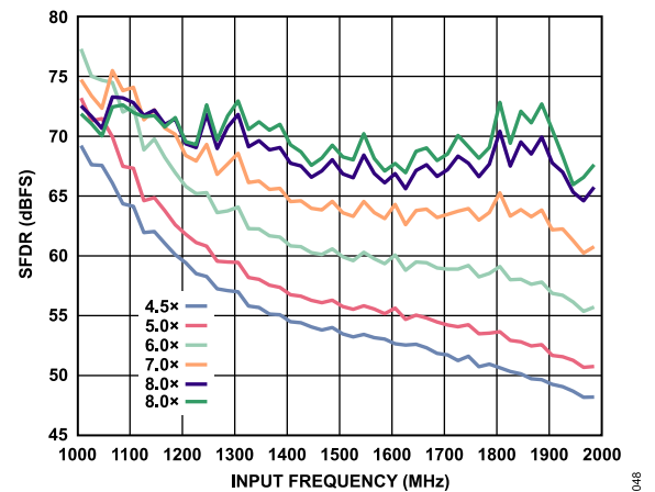
Figure 45. Buffer Current Sweeps (SFDR vs. Input Frequency and I_{BUFF} ), 1 GHz < f_{IN} < 2 GHz, Front-End Network Shown in Figure 40
