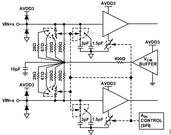
Figure 29. Analog Inputs
