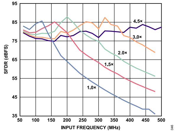
Figure 43. Buffer Current Sweeps (SFDR vs. Input Frequency and I_{BUFF} ), 10 MHz < f_{IN} < 500 MHz
