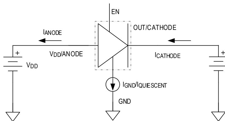
REVERSE-BIASED CONDITION
