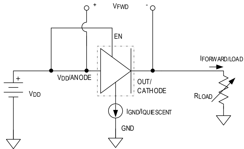
FORWARD-BIASED CONDITION
