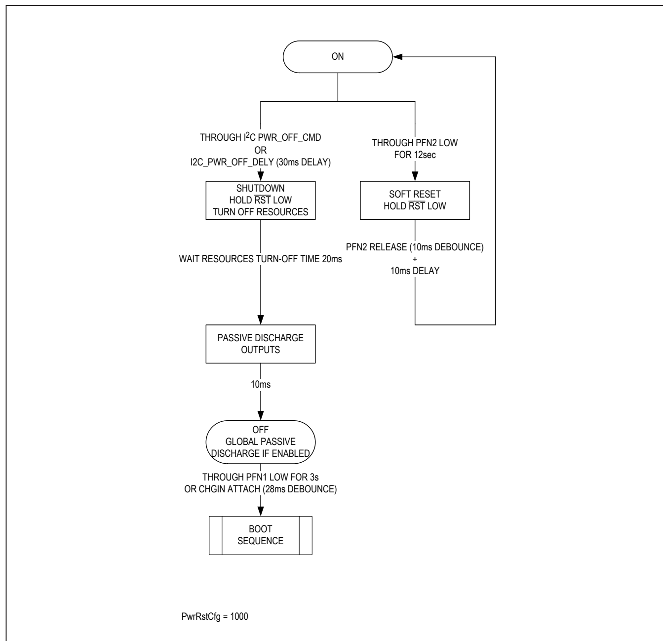
Figure 1f. PwrRstCfg = 1000
