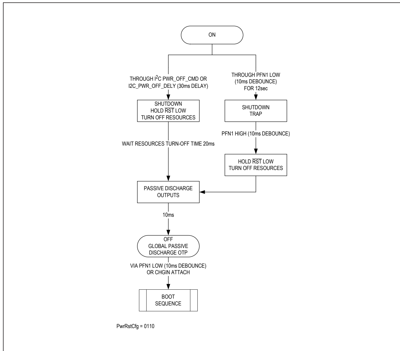
Figure 1d. PwrRstCfg = 0110
