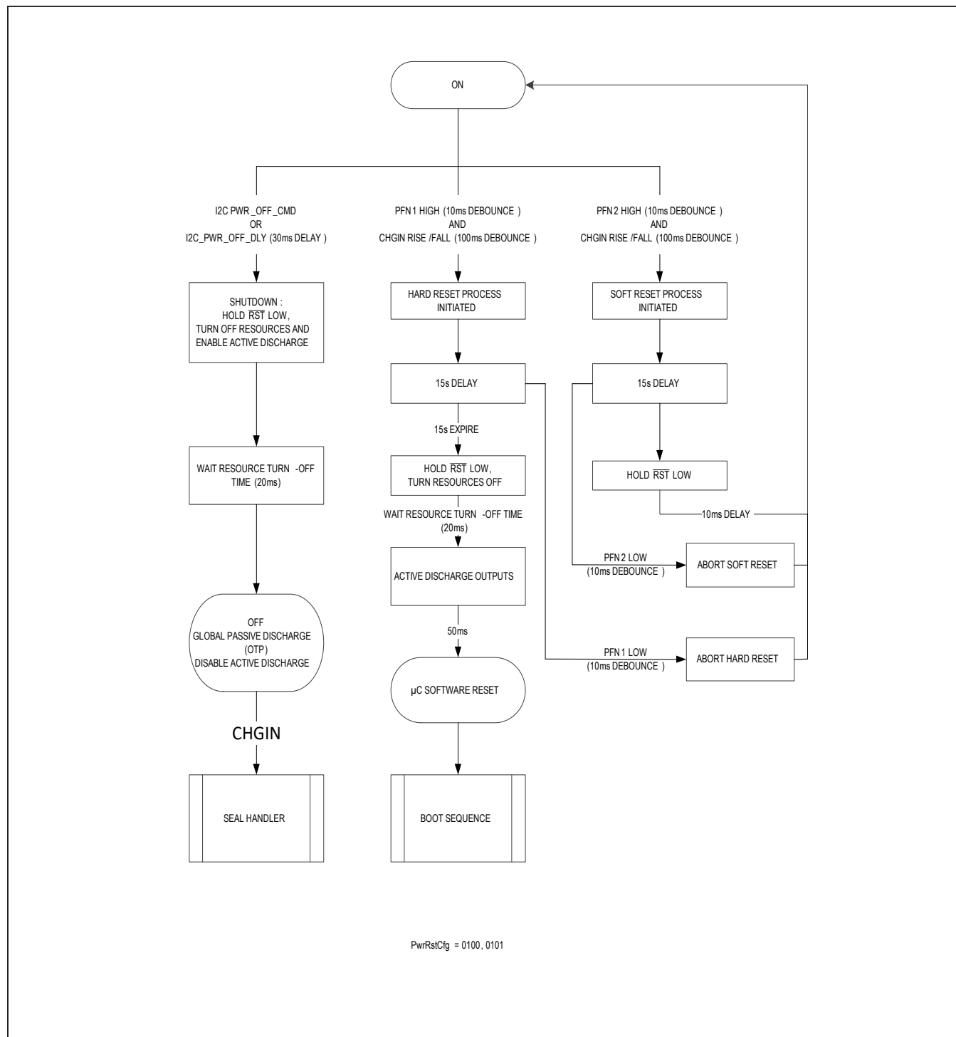
Figure 1c. PwrRstCfg = 0100 or 0101
