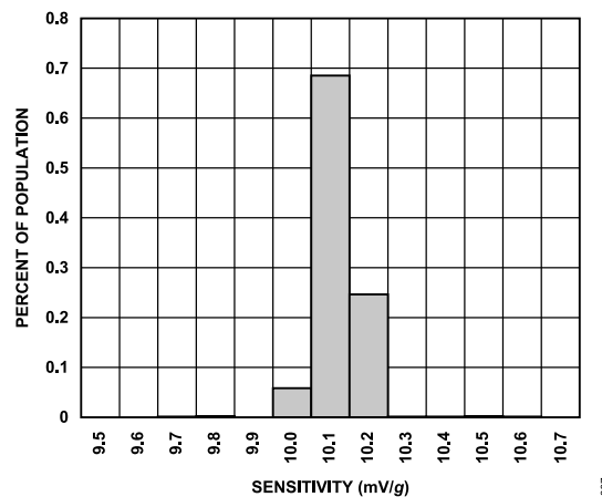
Figure 7. Sensitivity Distribution at 25°C
