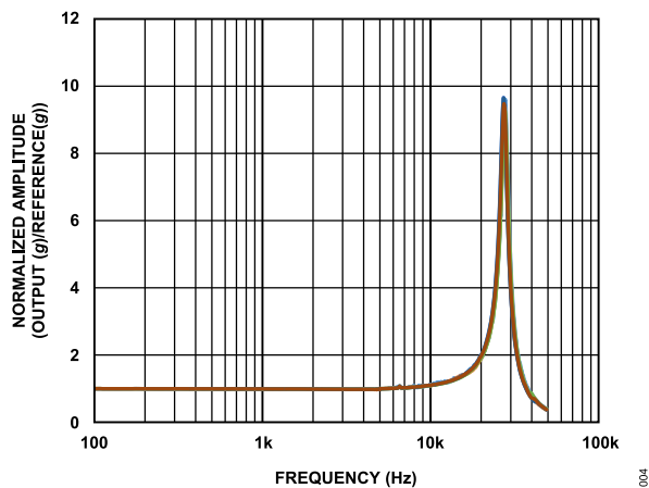
Figure 4. Frequency Response, High Frequency (>5 kHz) Vibration Response; a Laser Vibrometer Controller Referencing the ADXL1003 Package Used for Accuracy
