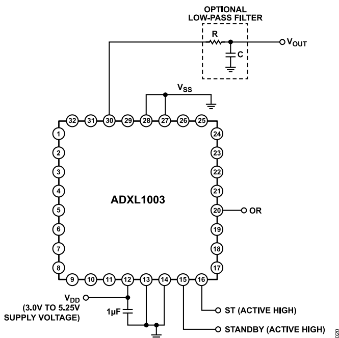
Figure 20. Application Circuit
