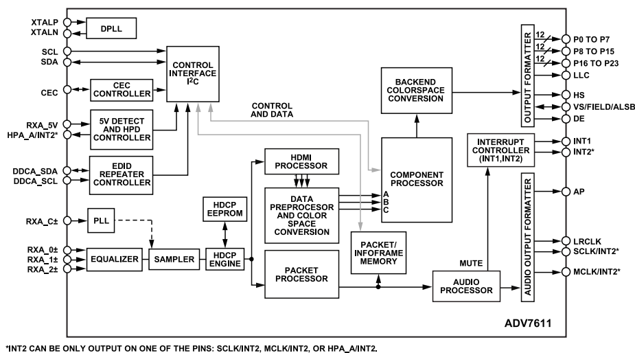
Figure 2. Detailed Functional Block Diagram
