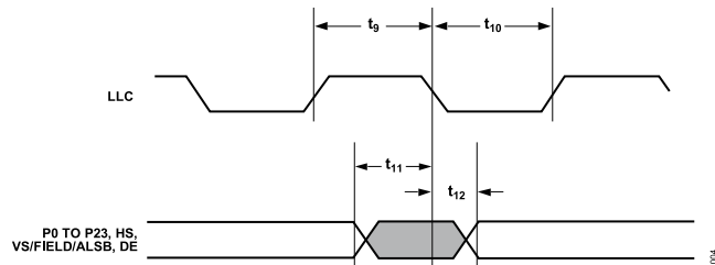
Figure 4. Pixel Port and Control SDR Output Timing
