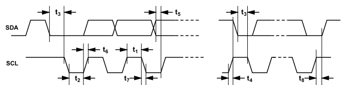
Figure 3. I 2 C Timing
