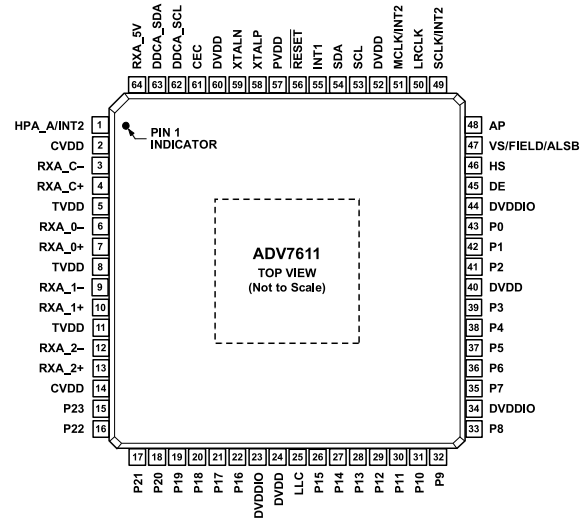
Figure 6. Pin Configuration
