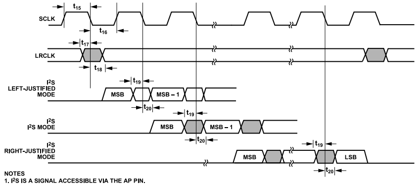
Figure 5. I 2 S Timing
