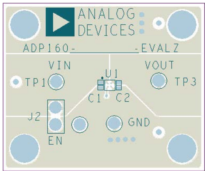
Figure 52. Example of 4-Ball WLCSP PCB Layout
