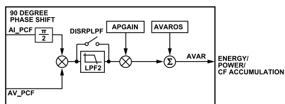
Figure 57. Total Reactive Power (AVAR) Calculation
