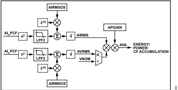
Figure 58. Total Apparent Power (AVA) Calculation
