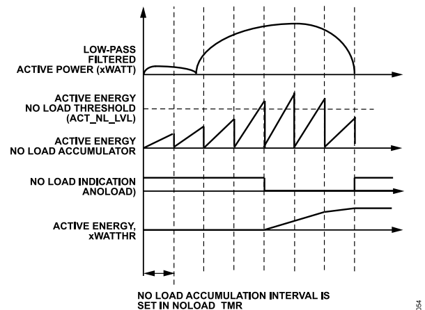
Figure 62. No Load Detection and Indication
