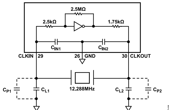
Figure 37. Crystal Application Circuit
