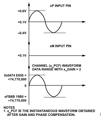
Figure 31. Maximum Input Signal with Pseudo Differential Input with Common-Mode Voltage = 0.1 V, Gain = 2
