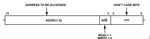
Figure 99. Command Header, CMD_HDR, Bits[15:0]
