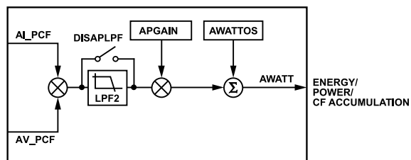
Figure 55. Total Active Power (AWATT) Calculation
