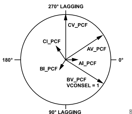
Figure 91. Phasor Diagram of xV\_PCF and xI\_PCF Waveforms Inside the IC with 3-Wire Delta with Phase B as Ground and VCONSEL = 001
