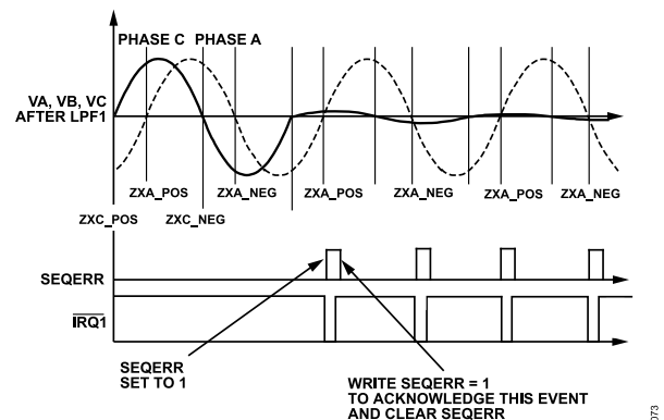
Figure 82. 3-Wire Delta Phase Sequence Error from a Phase Voltage Dropping Below ZXTHRS with SEQ_CYC = 1
