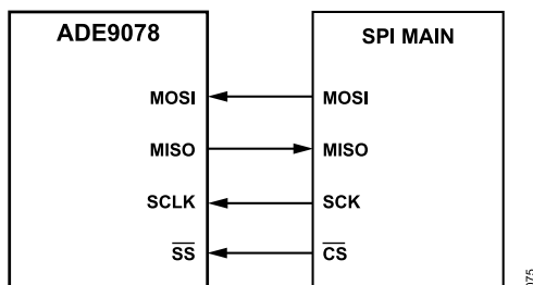
Figure 96. Connecting the ADE9078 Subordinate SPI Port to a Main SPI Device
