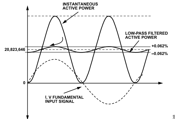
Figure 56. Instantaneous Active Power and Low-Pass Filtered Active Power at a Power Factor of 1
