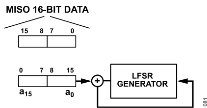
Figure 102. CRC Calculation of 16-Bit SPI Data
