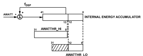
Figure 64. Internal Energy Register to AWATTHR_HI and AWATTHR_LO
