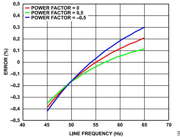
Figure 25. Total Active Energy Error as a Percentage of Reading vs. Line Frequency, Gain = 4, Integrator On
