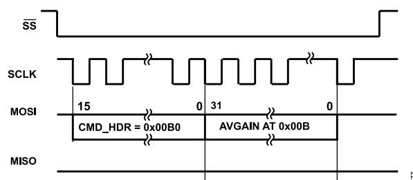
Figure 98. SPI Write Protocol Example
