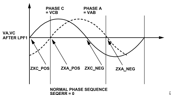
Figure 80. 3-Wire Delta Normal Phase Sequence
