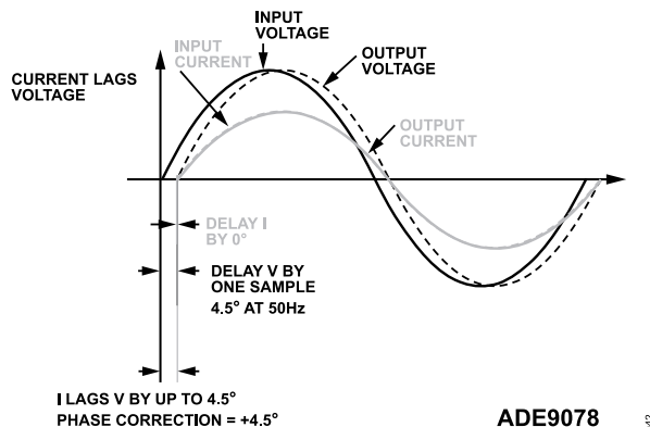
Figure 49. Phase Compensation Example Where Current Lags Voltage
