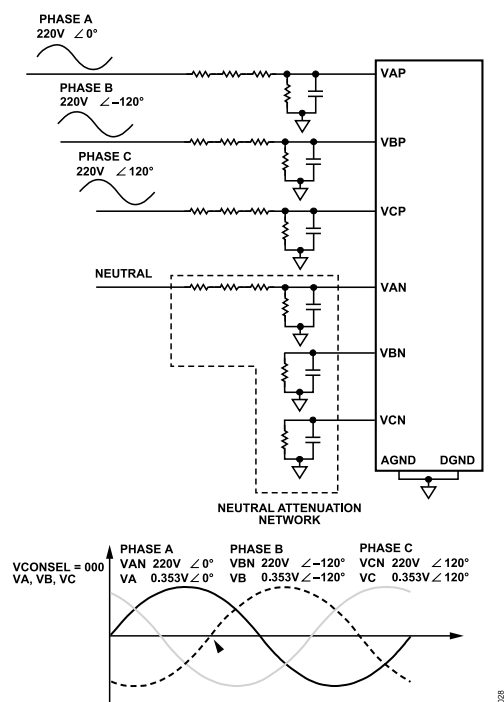
Figure 90. 4-Wire Wye, Series Impedance on the Neutral
