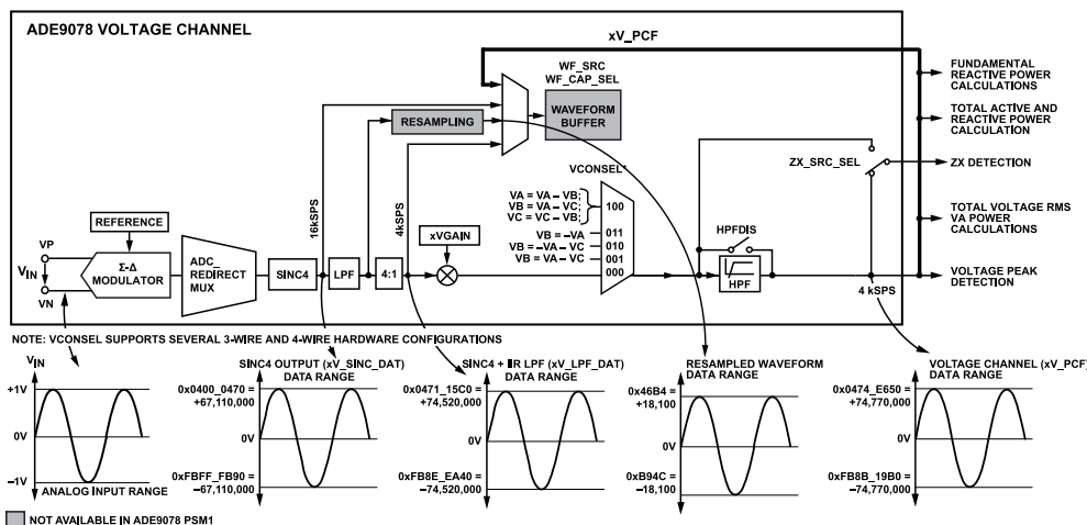
Figure 105. Voltage Channel Datapath
