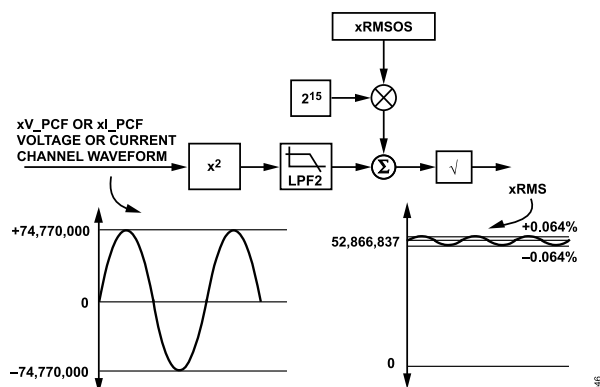
Figure 54. Filter Based RMS
