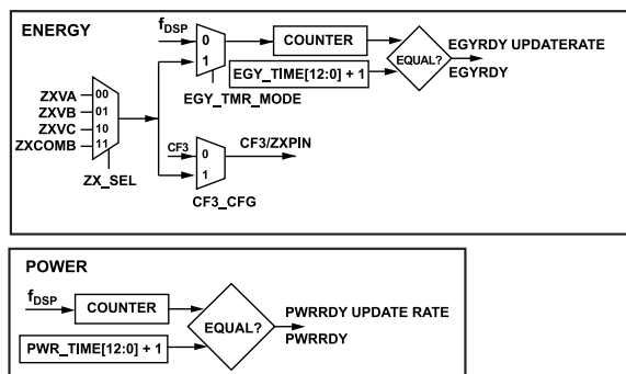
Figure 63. EGYRDY and PWRRDY Update Rates
