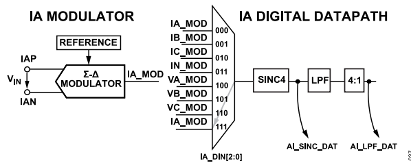
Figure 43. ADC_REDIRECT Modulator to Digital Datapath Multiplexing
