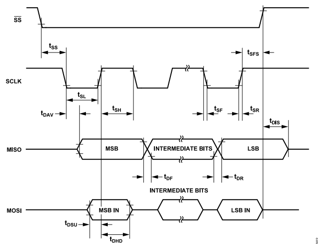
Figure 2. SPI Interface Timing
