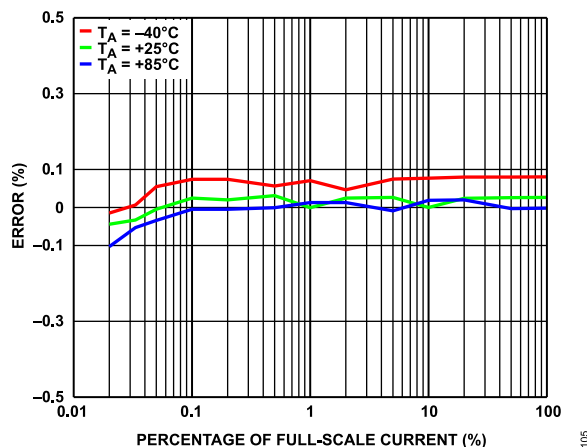
Figure 6. Total Apparent Energy Error as a Percentage of Reading over Temperature, PF = 1
