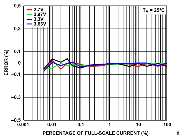
Figure 8. Total Reactive Energy Error as a Percentage of Reading over Supply Voltage, PF = 0 , T_A = 25^\circ
