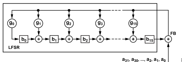
Figure 103. LFSR Generator Used for CRC_SPI Calculation
