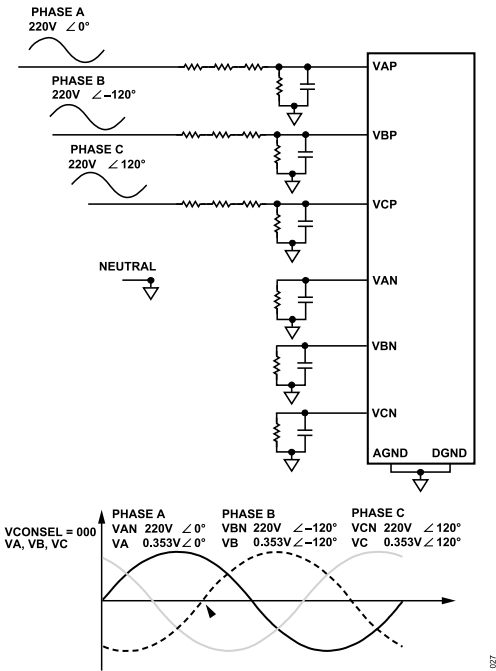
Figure 89. 4-Wire Wye, Neutral Connected to Ground
