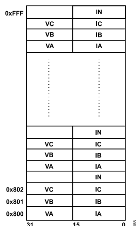
Figure 109. Resampled Waveform Sample Storage
