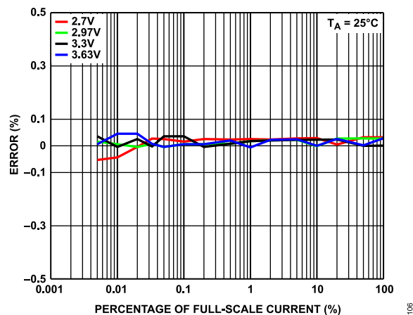
Figure 7. Total Active Energy Error as a Percentage of Reading over Supply Voltage, PF = 1, T_A = 25^\circ\text{C}
