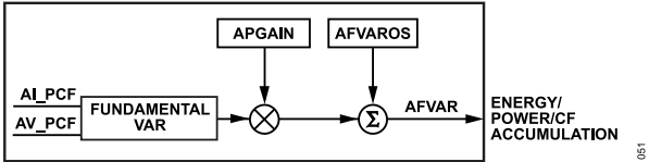
Figure 59. Fundamental Reactive Power, AFVAR
