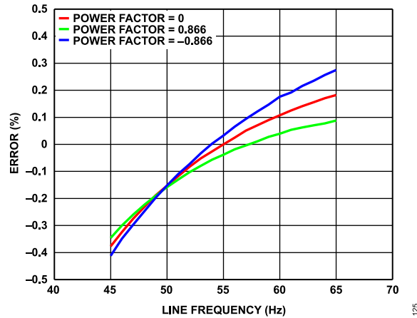
Figure 26. Total Reactive Energy Error as a Percentage of Reading vs. Line Frequency, Gain = 4, Integrator On
