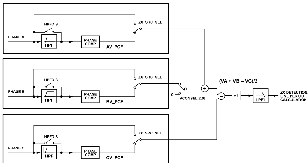
Figure 71. Combined Zero-Crossing Detection
