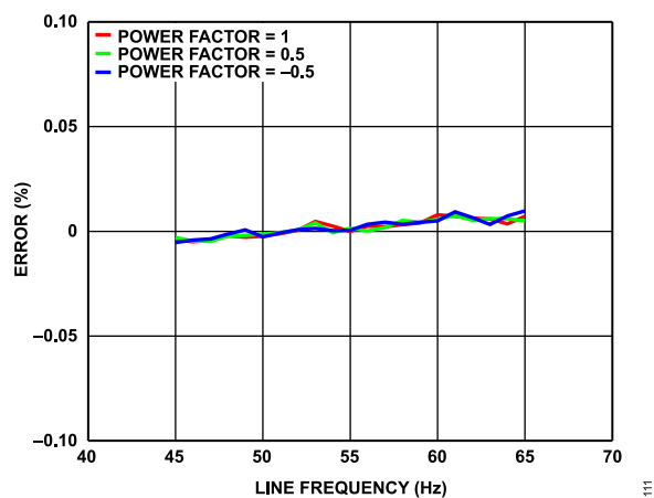
Figure 12. Total Active Energy Error as a Percentage of Reading vs. Line Frequency, PF = -0.5, +0.5, and +1
