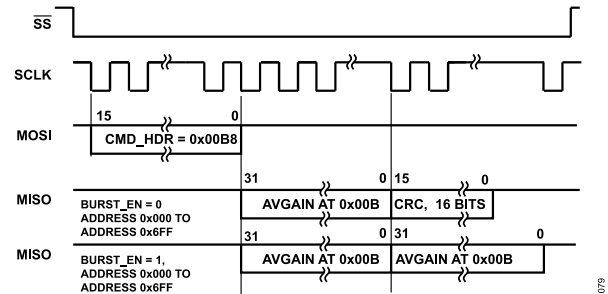
Figure 100. SPI Read Protocol Example Where the Following Data Is the CRC or the Initial Data Is Repeated
