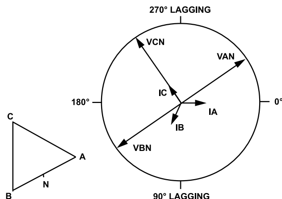
Figure 85. 4-Wire Delta Service Vector Diagram
