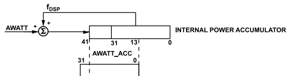
Figure 67. Internal Power Register to AWATT_ACC
