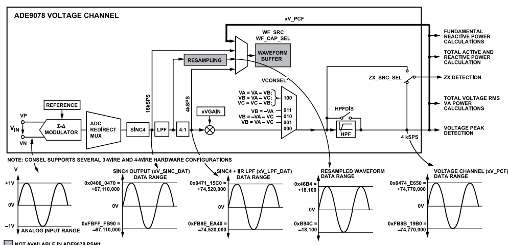
Figure 52. Voltage Channel Datapath
