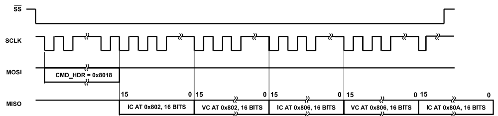
Figure 111. Waveform Buffer SPI Burst Read of Resampled Data, with BURST_CHAN = 0011 , to Read out IC and VC Data
