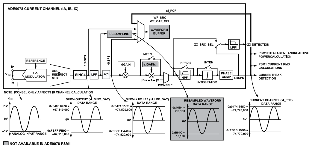
Figure 66. Current Channel PSM1 Datapath
