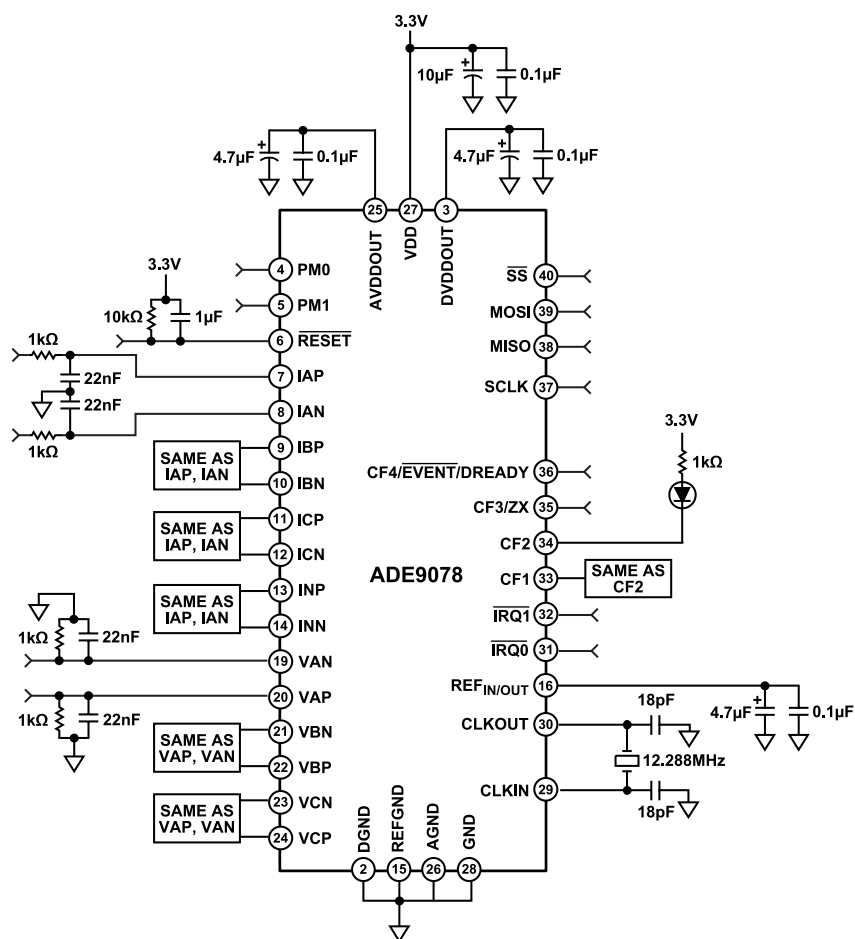
Figure 27. Test Circuit
