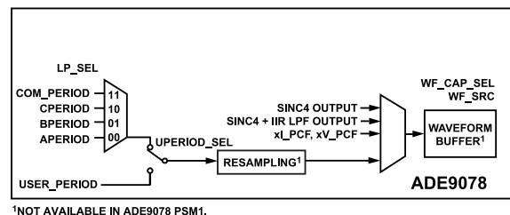
Figure 74. Line Period Selection for Resampling
