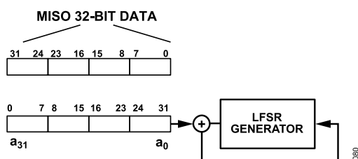
Figure 101. CRC Calculation of 32-Bit SPI Data
