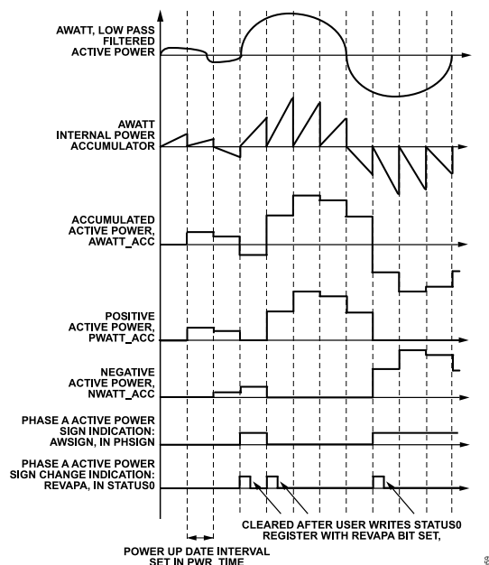
Figure 68. Power Accumulation and Power Sign
