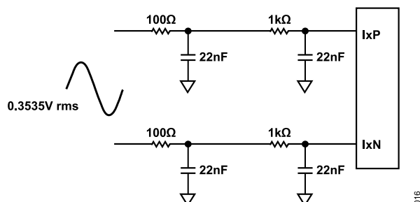
Figure 34. Application Circuit with Rogowski Coil Current Sensor
