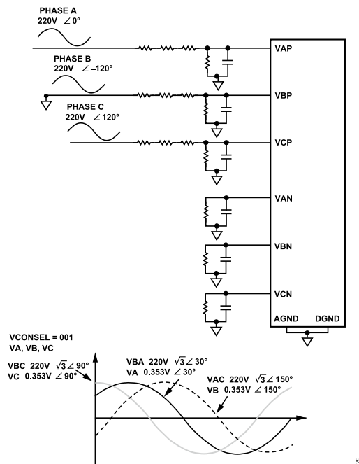
Figure 92. 3-Wire Delta, Phase B Connected to Ground
