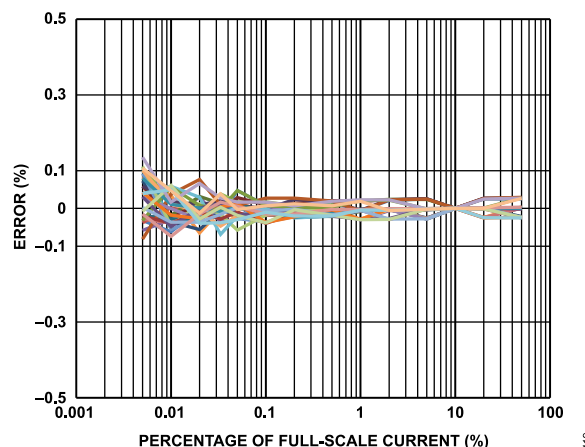
Figure 20. Fundamental Reactive Energy Error as a Percentage of Reading, PF = 0 (Standard Deviation \sigma = 0.04\% at 0.01% of Full-Scale Current)
