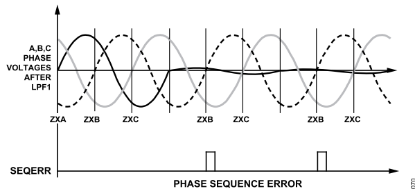
Figure 79. 4-Wire Wye, 4-Wire Delta Phase Sequence Error from a Phase Voltage Dropping Below ZXTHRS with SEQ_CYC = 1
