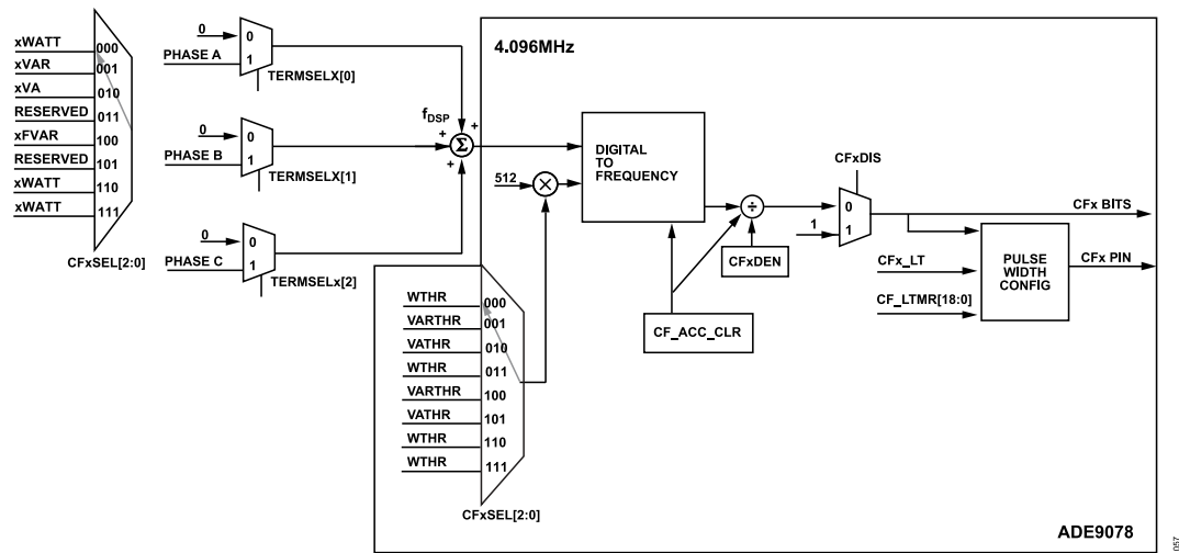
Figure 65. Digital to Frequency Conversion for CFx
