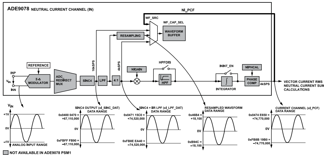
Figure 42. Neutral Current Channel Datapath
