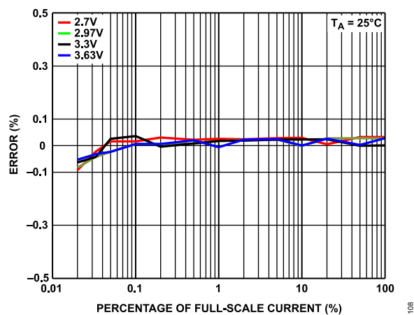
Figure 9. Total Apparent Energy Error as a Percentage of Reading over Supply Voltage, PF = 1 , T_A = 25^\circ
