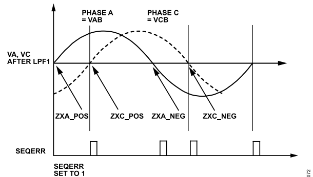
Figure 81. 3-Wire Delta Phase Sequence Error (Wiring Error)
