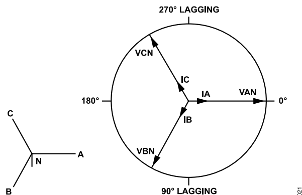
Figure 83. 4-Wire Wye Service Vector Diagram
