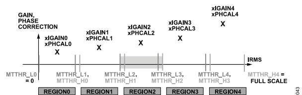
Figure 50. Multipoint Gain and Phase Calibration
