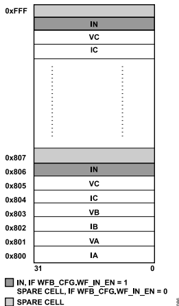
Figure 107. Fixed Data Rate Waveform Sample Storage
