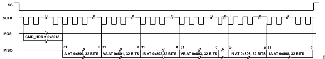
Figure 110. Waveform Buffer SPI Burst Read of Fixed Data Rate Samples, with BURST_CHAN = 0000, to Read out All Channels (the Default State of the MOSI Pin Depends on the Main SPI Device; It Is Assumed to Be High (Logic 1))
