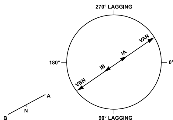
Figure 86. 3-Wire Residential Single-Phase Service Vector Diagram
