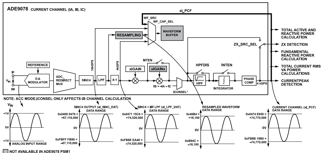
Figure 41. Current Channel Datapath
