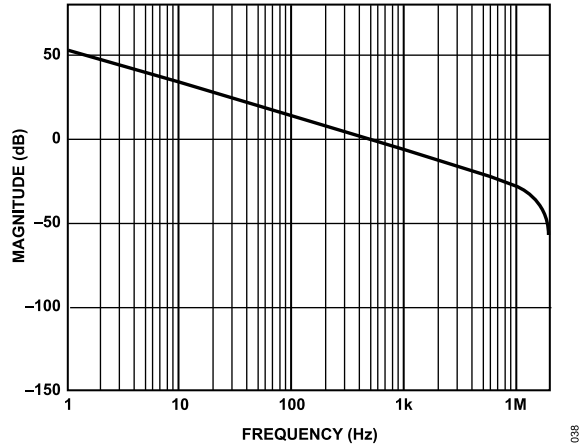
Figure 44. Digital Integrator Magnitude Response, DICOEFF = 0xFFFFE000
