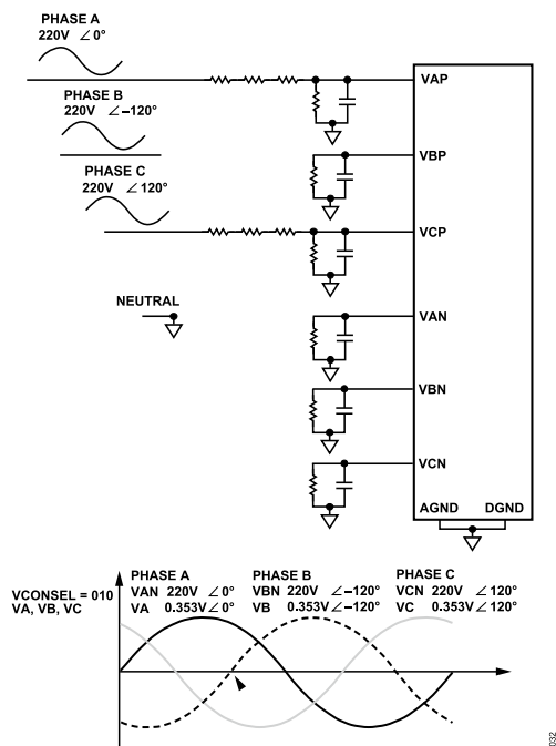
Figure 94. Non-Blondel Compliant 4-Wire Wye
