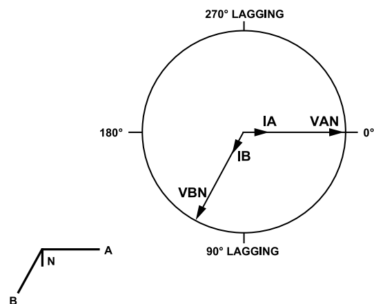
Figure 87. 3-Wire Network Meter Vector Diagram
