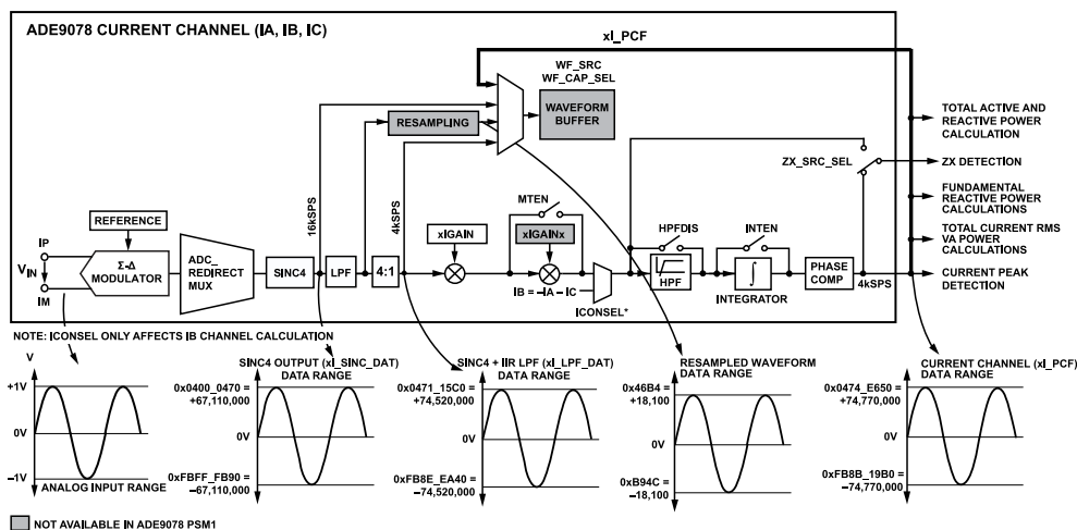
Figure 104. Current Channel Datapath
