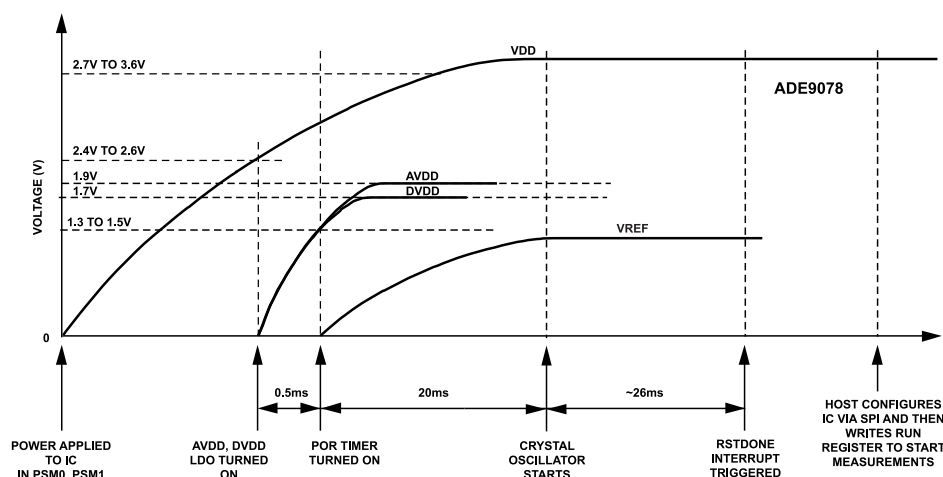
Figure 39. Power-On Sequence for PSM0 and PSM1
