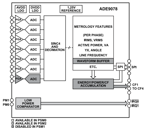
Figure 40. Features Available in Each Operating Mode
