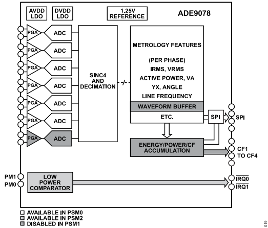
Figure 38. Functions Available in PSM1 and PSM2
