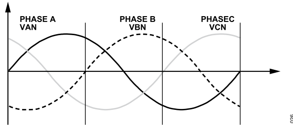
Figure 88. 4-Wire Wye, Voltage Phase Sequence in Time
