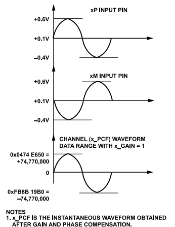
Figure 30. Maximum Input Signal with Differential Antiphase Input with Common-Mode Voltage = 0.1 V, Gain = 1
