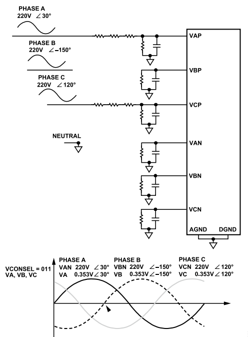
Figure 95. Non-Blondel Compliant 4-Wire Delta
