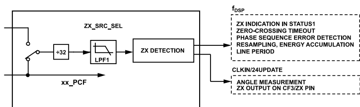
Figure 72. Zero-Crossing Output Rates
