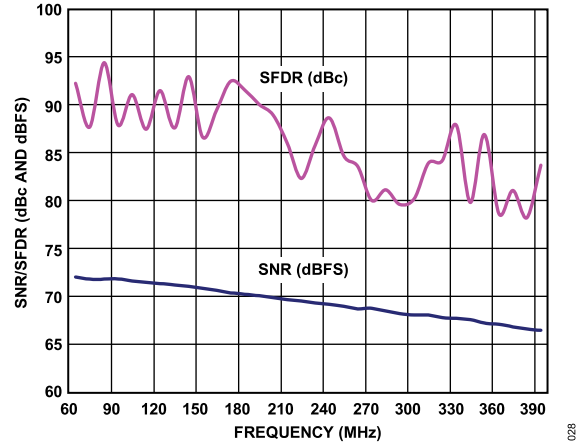
Figure 21. AD9643-210 Single-Tone SNR/SFDR vs. Input Frequency ( f_{IN} )
