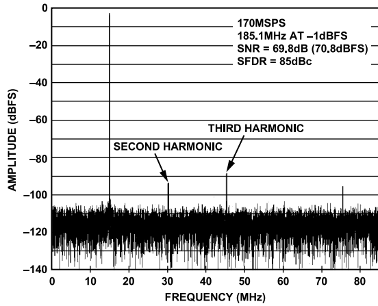
Figure 7. AD9643-170 Single-Tone FFT with f_{IN} = 185.1 MHz
