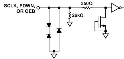
Figure 43. Equivalent SCLK, PDWN, or OEB Input Circuit
