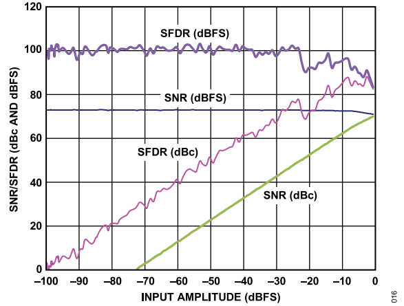
Figure 9. AD9643-170 Single-Tone SNR/SFDR vs. Input Amplitude ( A_{IN} ) with f_{IN} = 90.1 MHz
