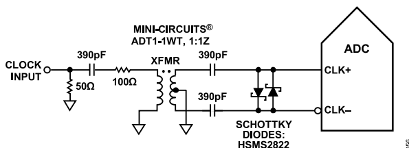
Figure 52. Transformer-Coupled Differential Clock (Up to 200 MHz)
