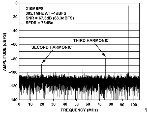
Figure 19. AD9643-210 Single-Tone FFT with f_{IN} = 305.1 MHz
