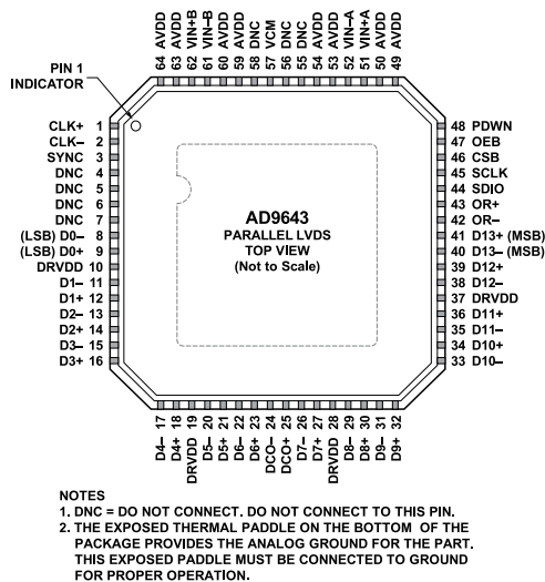
Figure 4. LFCSP Interleaved Parallel LVDS Pin Configuration (Top View)
