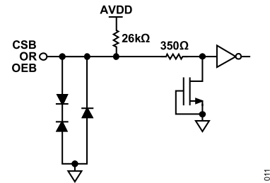
Figure 44. Equivalent CSB Input Circuit
