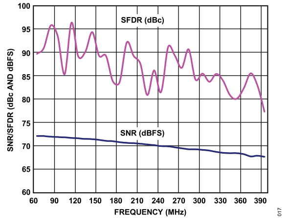
Figure 10. AD9643-170 Single-Tone SNR/SFDR vs. Input Frequency ( f_{IN} )
