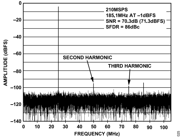
Figure 18. AD9643-210 Single-Tone FFT with f_{IN} = 185.1 MHz
