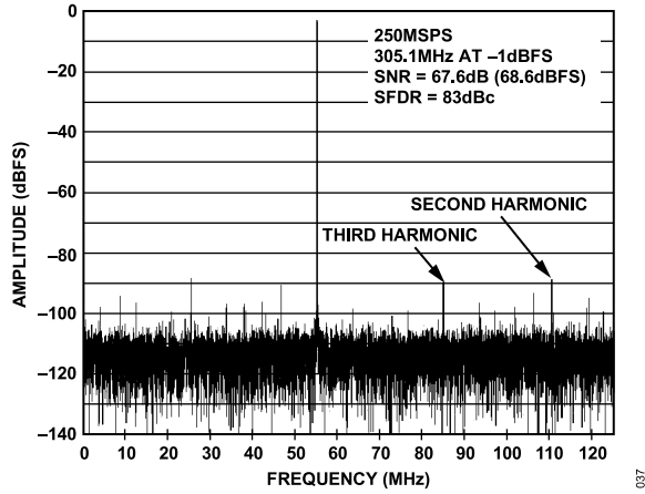
Figure 30. AD9643-250 Single-Tone FFT with f_{IN} = 305.1 MHz
