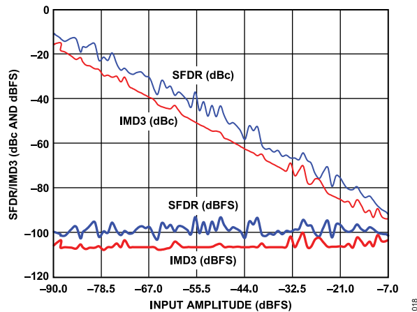
Figure 11. AD9643-170 Two-Tone SFDR/IMD3 vs. Input Amplitude ( A_{IN} ) with f_{IN1} = 89.12 , f_{IN2} = 92.12 MHz, f_s = 170 MSPS
