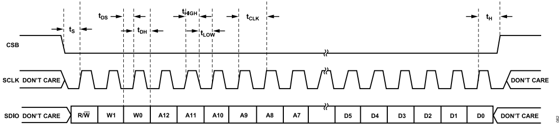
Figure 58. Serial Port Interface Timing Diagram
