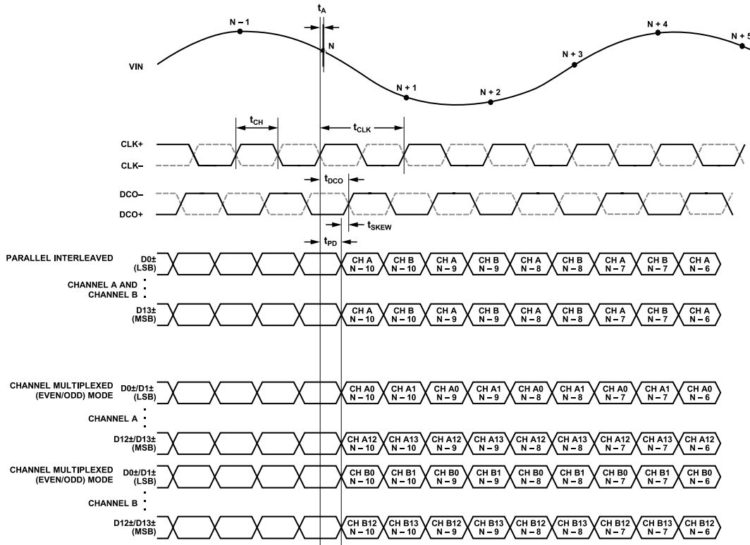
Figure 2. LVDS Modes for Data Output Timing
