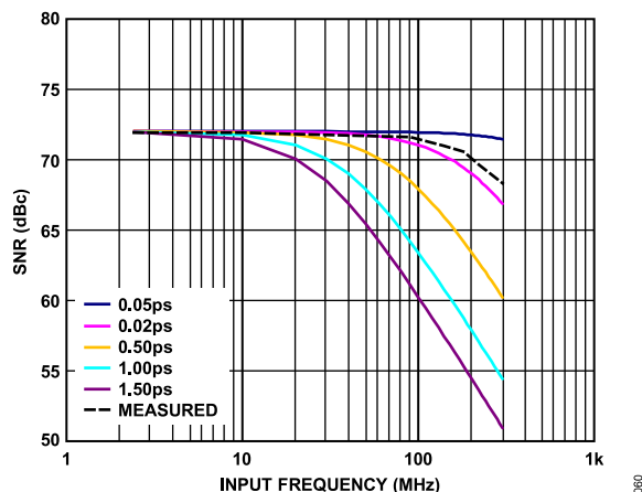
Figure 56. AD9643-250 SNR vs. Input Frequency and Jitter
