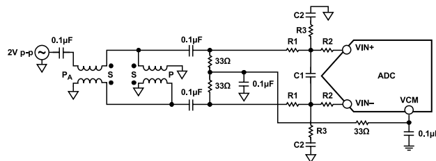
Figure 50. Differential Double Balun Input Configuration
