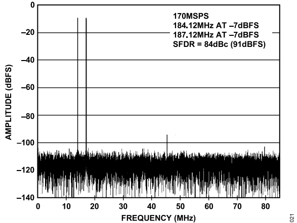
Figure 14. AD9643-170 Two-Tone FFT with f_{IN1} = 184.12 , f_{IN2} = 187.12 MHz, f_S = 170 MSPS
