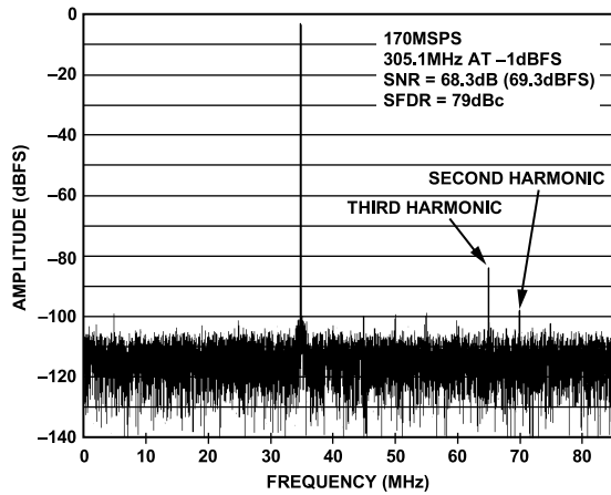
Figure 8. AD9643-170 Single-Tone FFT with f_{IN} = 305.1 MHz
