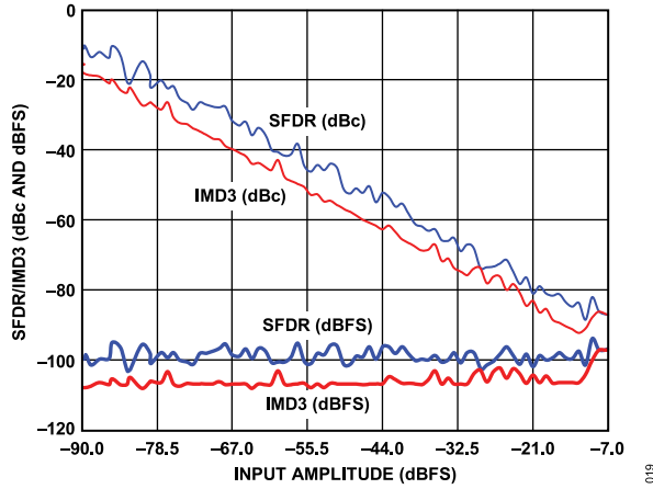
Figure 12. AD9643-170 Two-Tone SFDR/IMD3 vs. Input Amplitude ( A_{IN} ) with f_{IN1} = 184.12 , f_{IN2} = 187.12 MHz, f_S = 170 MSPS
