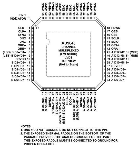
Figure 5. LFCSP Channel Multiplexed (Even/Odd) LVDS Pin Configuration (Top View)
