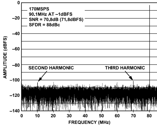
Figure 6. AD9643-170 Single-Tone FFT with f_{IN} = 90.1 MHz
