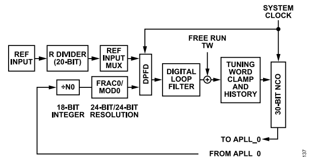
Figure 31. DPLL_0 Core
