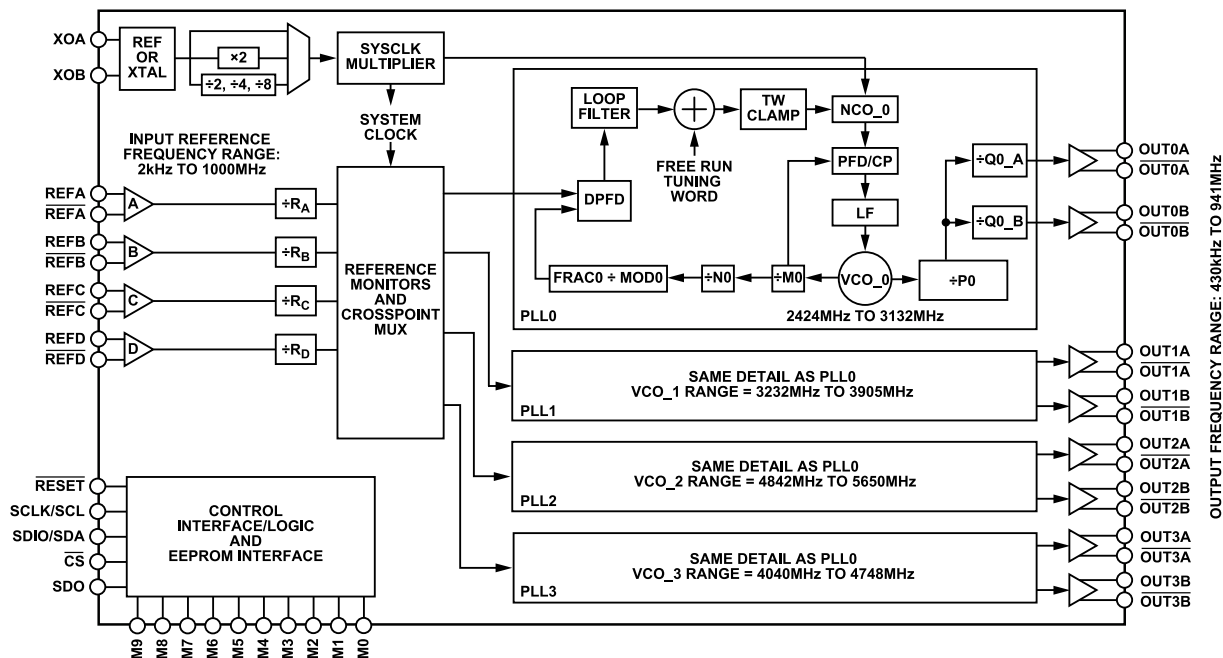
Figure 30. Detailed Block Diagram
