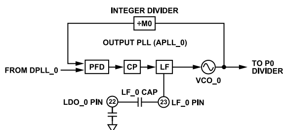
Figure 34. APLL_0 Block Diagram
