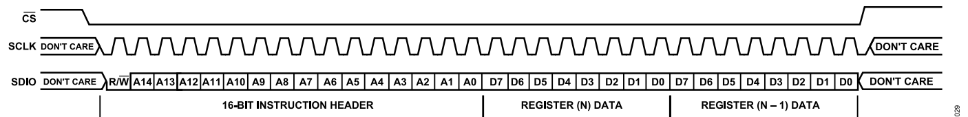
Figure 37. Serial Control Port Write—MSB First, Address Decrement, Two Bytes of Data
