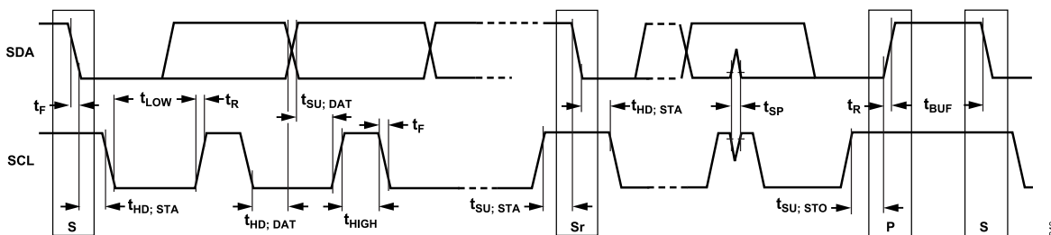
Figure 48. I 2 C Serial Port Timing
