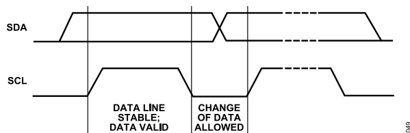
Figure 43. Valid Bit Transfer
