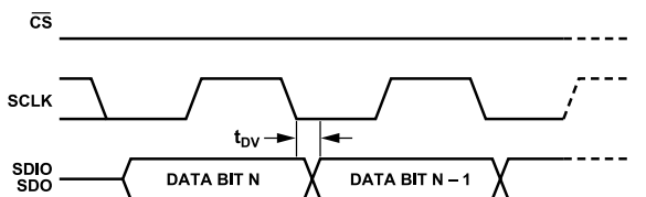
Figure 40. Timing Diagram for Serial Control Port Register Read—MSB First
