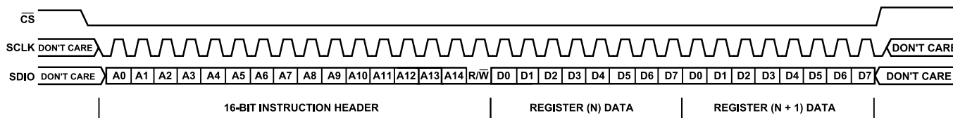
Figure 41. Serial Control Port Write—LSB First, Address Increment, Two Bytes of Data
