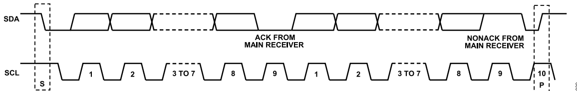
Figure 47. Data Transfer Process (Main Read Mode, 2-Byte Transfer), First Acknowledge From Node
