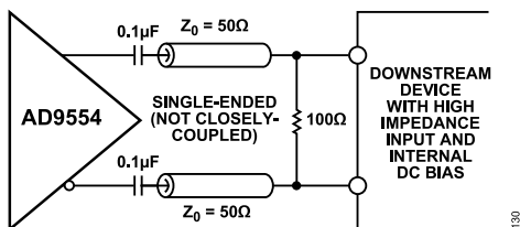
Figure 21. Destination Self-Biased Differential Receiver; Use 14 mA Mode for LVDS-Compatible Amplitude or 28 mA for LVPECL-Compatible Amplitudes (100 Ω resistor must be as close to the destination receiver as possible.)
