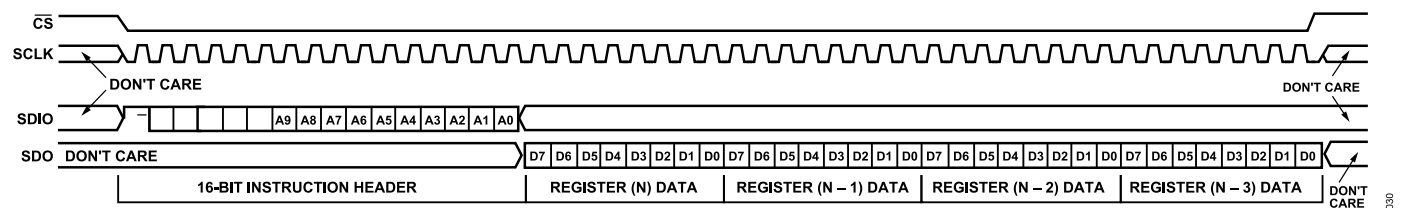
Figure 38. Serial Control Port Read—MSB First, Address Decrement, Four Bytes of Data
