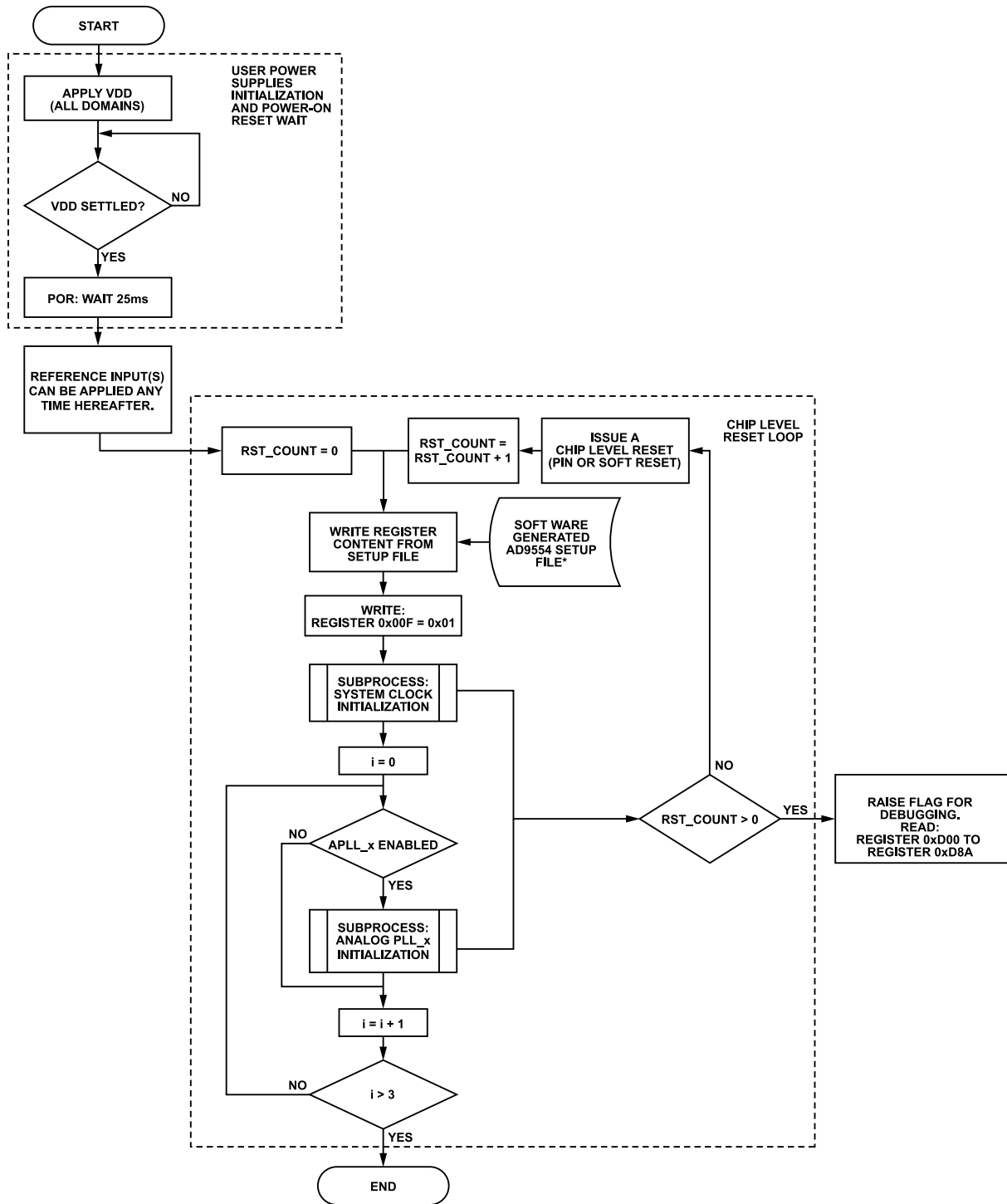
Figure 26. Main Process—Initialization
