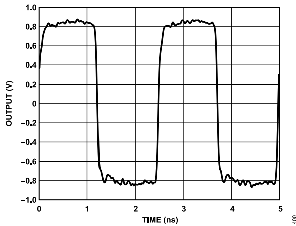
Figure 14. Output Waveform, 28 mA LVPECL-Compatible Mode (400 MHz) with 100 Ω Termination Resistor
