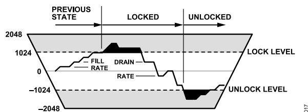
Figure 33. Lock Detector Diagram
