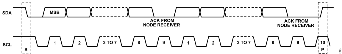
Figure 46. Data Transfer Process (Main Write Mode, 2-Byte Transfer)
