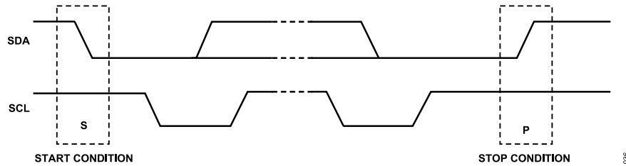
Figure 44. Start and Stop Conditions
