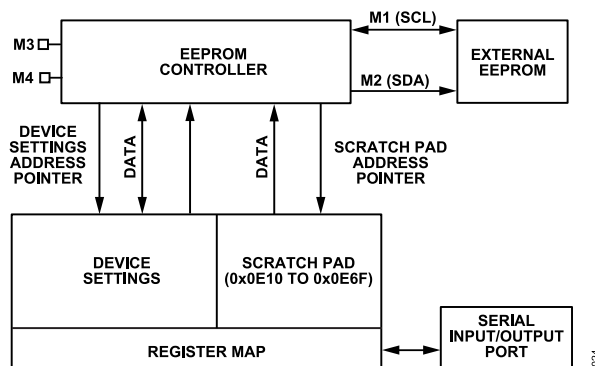
Figure 36. EEPROM Functional Diagram
