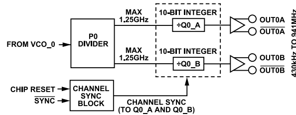
Figure 35. Clock Distribution Block Diagram from VCO_0 for the PLL_0
