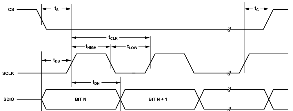
Figure 42. Serial Control Port Timing—Write
