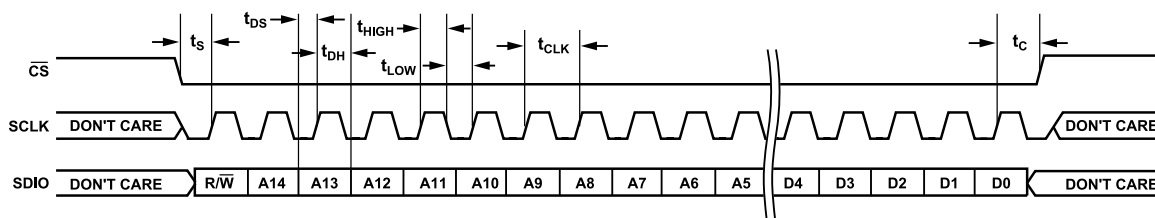
Figure 39. Timing Diagram for Serial Control Port Write—MSB First
