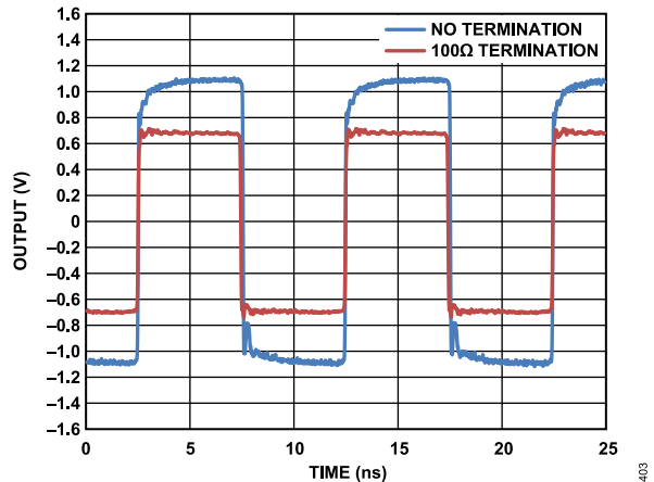
Figure 17. Output Waveform, 21 mA Mode (100 MHz)
