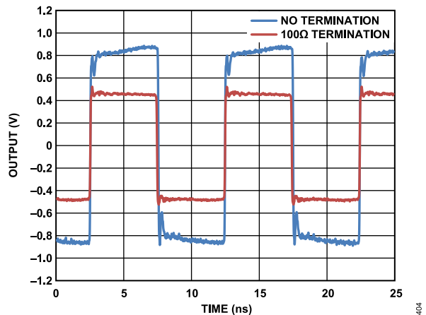
Figure 18. Output Waveform, 14 mA Mode (100 MHz)
