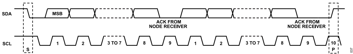
Figure 45. Acknowledge Bit
