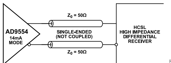
Figure 22. DC-Coupled HCSL Receiver
