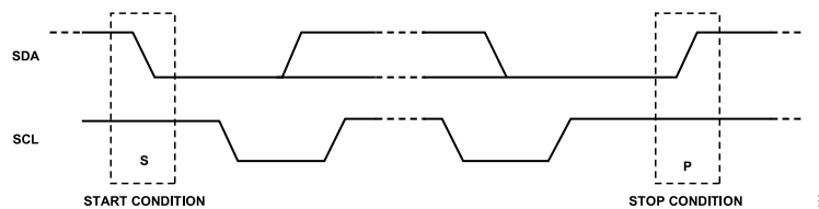
Figure 63. Start and Stop Conditions
