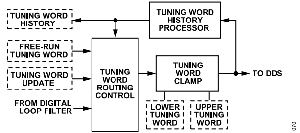
Figure 46. Tuning Word Processing
