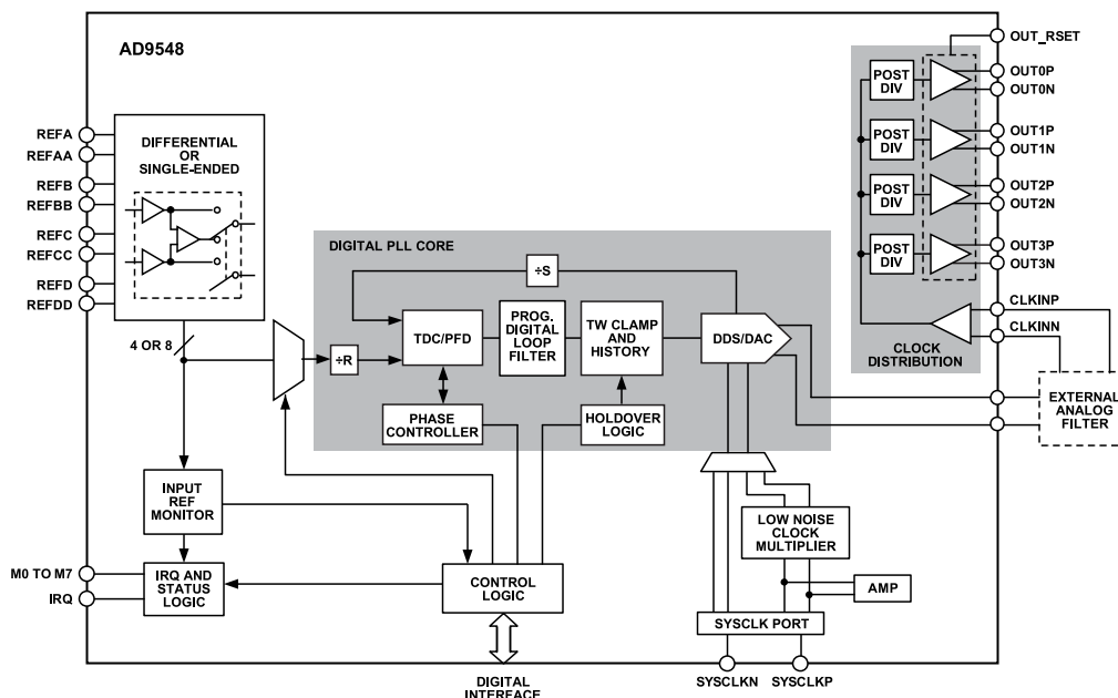
Figure 35. Detailed Block Diagram
