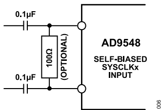
Figure 31. SYSCLKx Input
