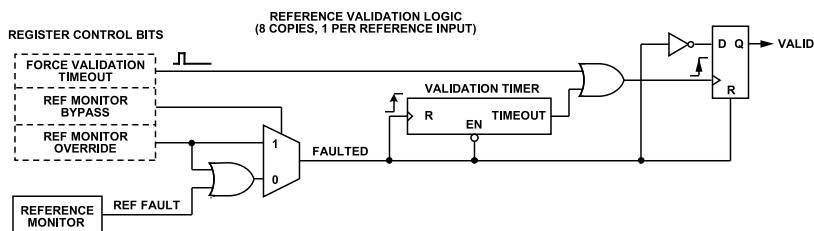
Figure 36. Reference Validation Override
