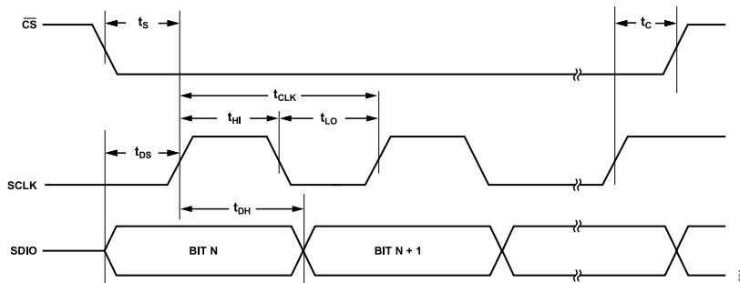
Figure 61. Serial Control Port Timing—Write
