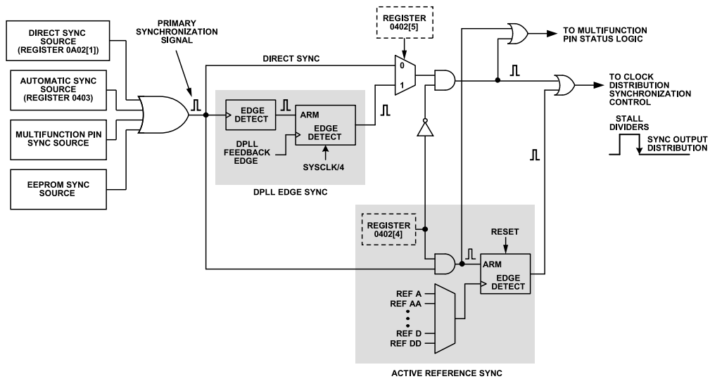
Figure 50. Output Synchronization Block Diagram
