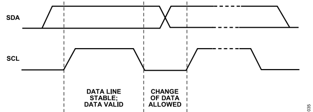
Figure 62. Valid Bit Transfer
