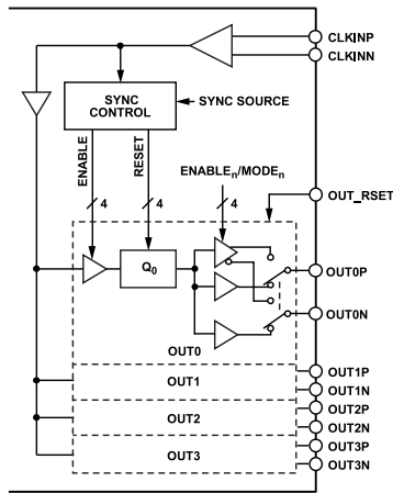
Figure 49. Clock Distribution
