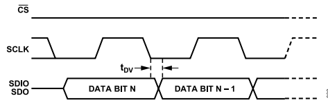
Figure 59. Timing Diagram for Serial Control Port Register Read
