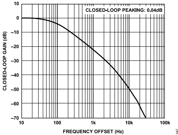
Figure 16. Jitter Transfer Bandwidth, Output Driver = LVPECL, f_R = 19.44 MHz, f_0 = 155.52 MHz, LBW = 100 Hz (Phase Margin = 88°), f_{SYS} = 1 GHz, PLL Off
