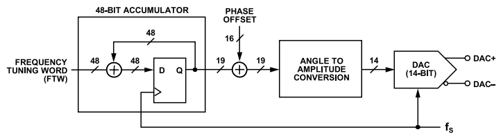
Figure 44. DDS Block Diagram
