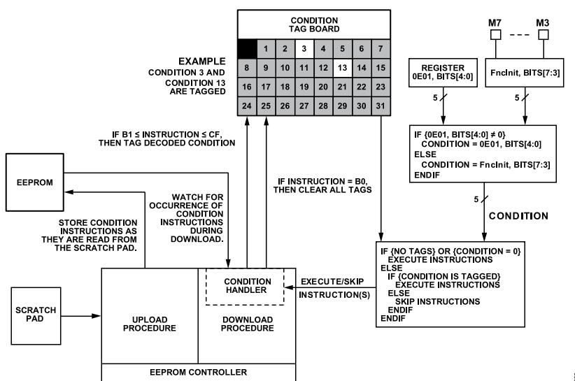
Figure 52. EEPROM Conditional Processing
