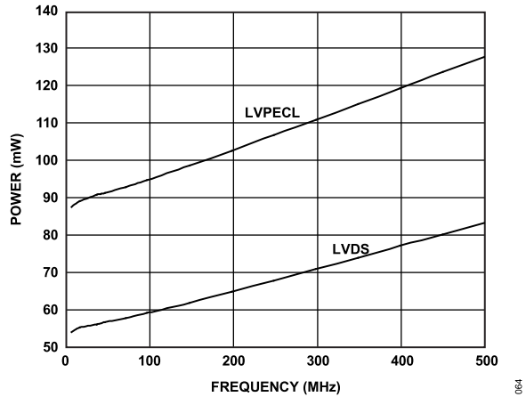
Figure 19. Power Consumption vs. Frequency, LVPECL and LVDS (Single Channel)
