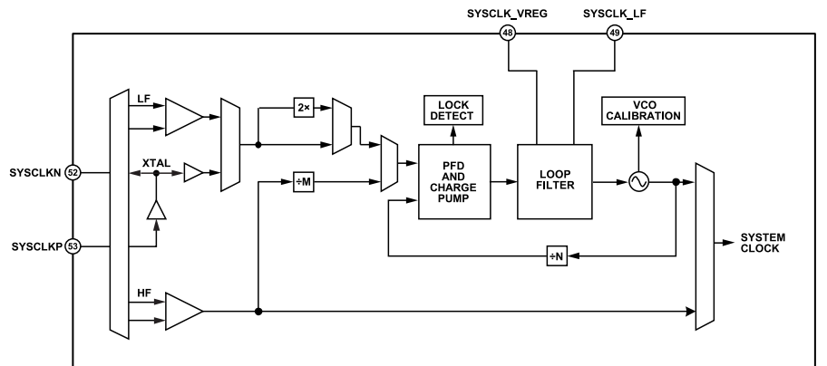
Figure 47. System Clock Block Diagram
