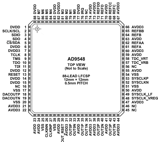
Figure 2. 88-Lead LFCSP Pin Configuration
