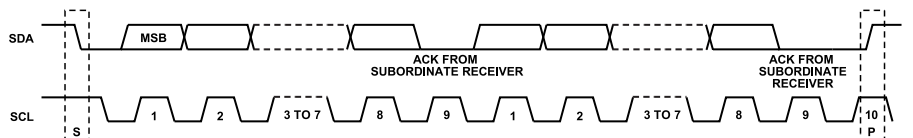
Figure 64. Acknowledge Bit
