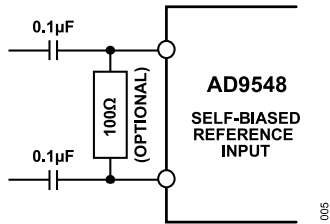
Figure 30. Reference Input
