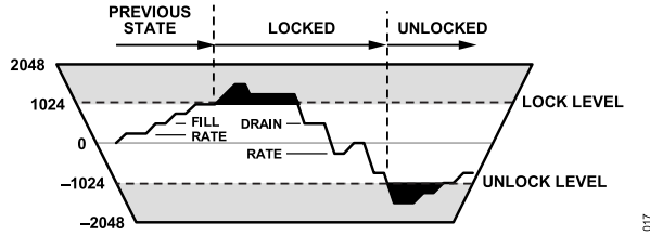
Figure 43. Lock Detector Diagram
