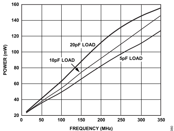
Figure 20. Power Consumption vs. Frequency, 3.3 V CMOS (Strong Mode)
