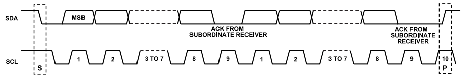
Figure 65. Data Transfer Process (Main Write Mode, 2-Byte Transfer)
