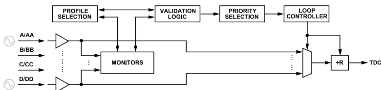
Figure 38. Reference Clock Block Diagram
