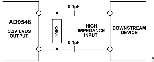
Figure 28. AC-Coupled LVDS or LVPECL Output Driver
