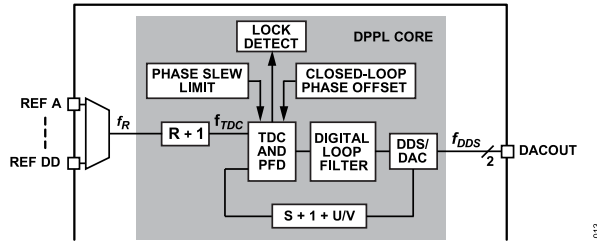
Figure 39. Digital PLL Core
