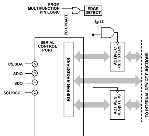
Figure 68. Buffered and Active Registers
