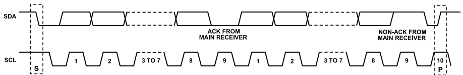
Figure 66. Data Transfer Process (Main Read Mode, 2-Byte Transfer)
