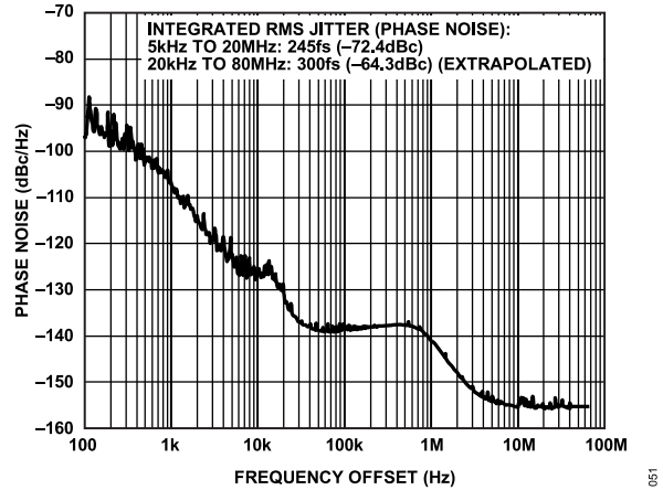
Figure 12. Absolute Phase Noise (Output Driver = LVPECL), f_R = 19.44 \text{ MHz} , f_O = 155.52 \text{ MHz} , LBW = 1 \text{ kHz} , f_{SYS} = 50 \text{ MHz} (Crystal), PLL On with 2x Frequency Multiplier, I_{CP} = 375 \mu\text{A} , LF = \text{External (350 kHz)}
