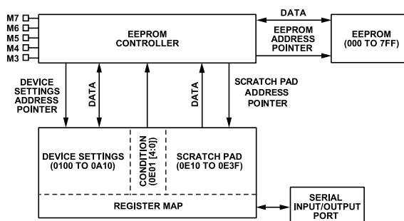
Figure 51. EEPROM Functional Diagram
