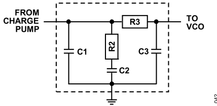
Figure 69. Third Order Analog Loop Filter
