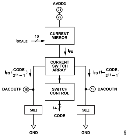
Figure 45. DAC Output Pins
