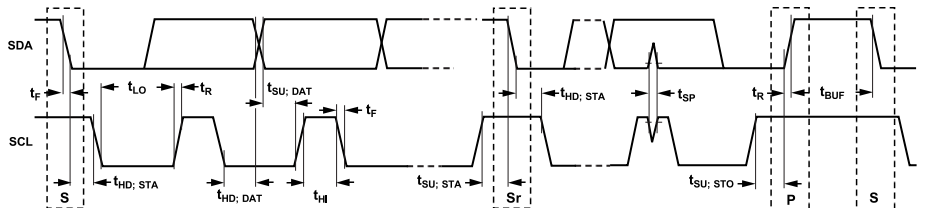
Figure 67. I 2 C Serial Port Timing
