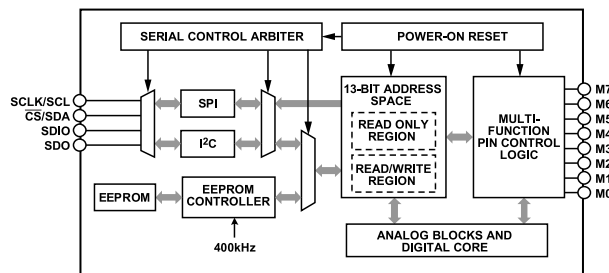
Figure 53. Serial Port Functional Diagram
