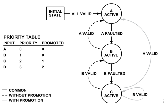
Figure 37. Example of Priority Promotion
