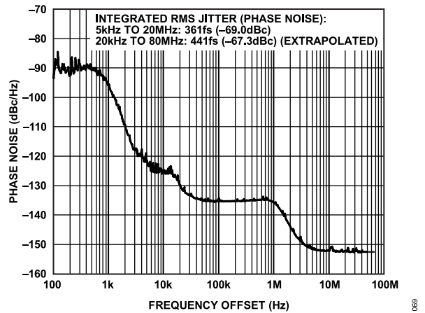
Figure 7. Absolute Phase Noise (Output Driver = LVPECL), f_R = 19.44 MHz, f_O = 155.52 MHz, LBW = 1 kHz, f_{SYS} = 50 MHz, PLL On
