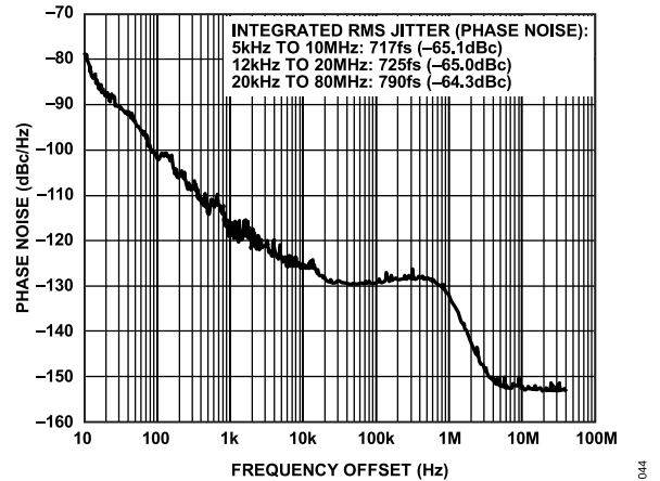
Figure 8. Absolute Phase Noise (Output Driver = LVPECL), f_R = 1 Hz, f_O = 122.88 MHz, LBW = 0.05 Hz, f_{SYS} = 20 MHz (OCXO), PLL On
