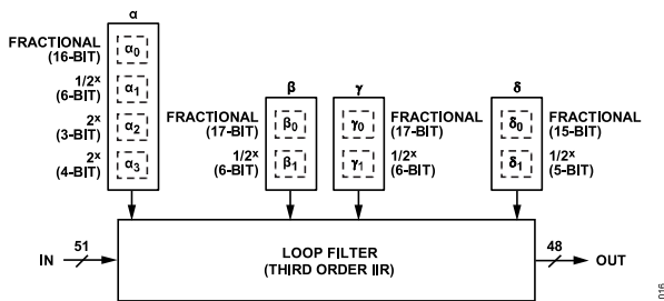
Figure 42. Third Order Digital IIR Loop Filter
