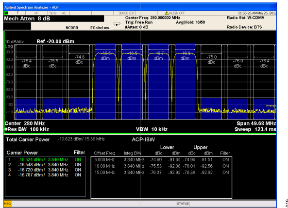
Figure 22. 4C WCDMA ACLR Performance, f_c = 280 MHz, f_{DAC} = 1474.28 MHz
