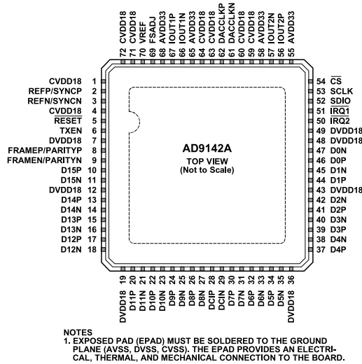
Figure 2. Pin Configuration
