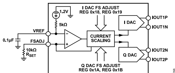
Figure 56. Simplified Block Diagram of DAC Core
