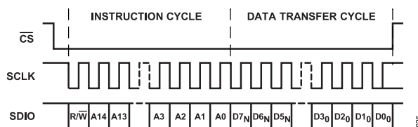
Figure 29. Serial Register Interface Timing, MSB First
