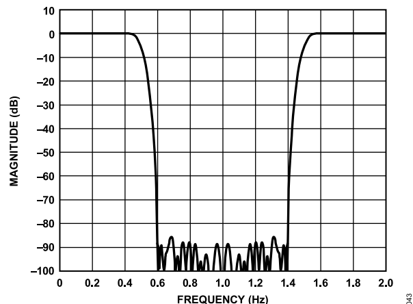
Figure 42. All-Band Response of 2\times Mode
