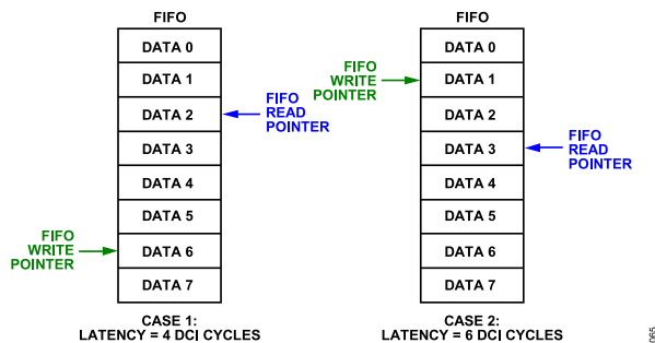
Figure 63. Example of FIFO Latency Difference
