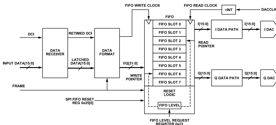
Figure 39. Block Diagram of FIFO
