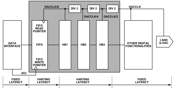
Figure 62. Breakdown of Pipeline Latencies
