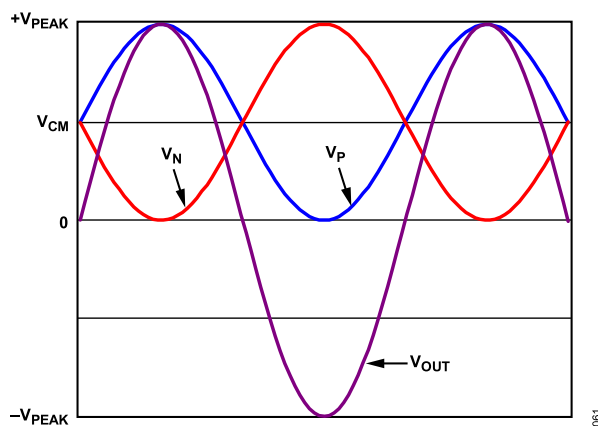
Figure 59. Output Voltage Waveforms
