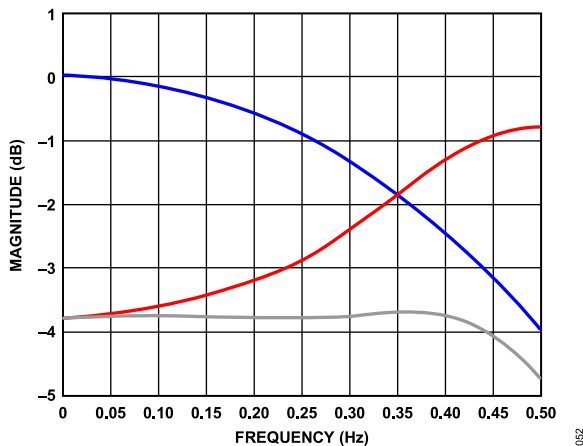
Figure 49. Responses of \sin(x)/x Roll Off (Blue), the \text{Sinc}^{-1} Filter (Red), and Composite of Both (Black)
