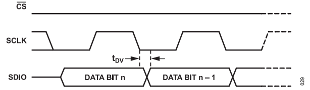
Figure 32. Timing Diagram for Serial Port Register Read
