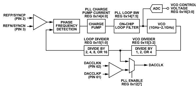
Figure 54. PLL Clock Multiplication Circuit
