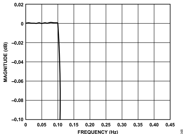
Figure 45. Pass-Band Detail of 8x Mode
