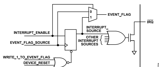
Figure 51. Simplified Schematic of \overline{\text{IRQ}} Circuitry
