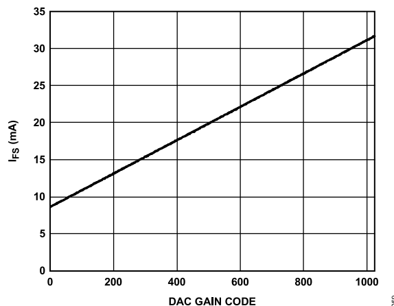
Figure 57. DAC Full-Scale Current vs. DAC Gain Code
