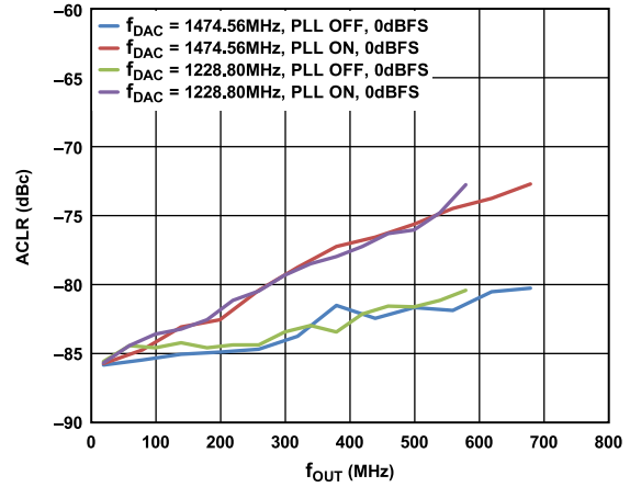
Figure 18. 1C WCDMA, Second Adjacent ACLR vs. f_{OUT} , PLL On and Off
