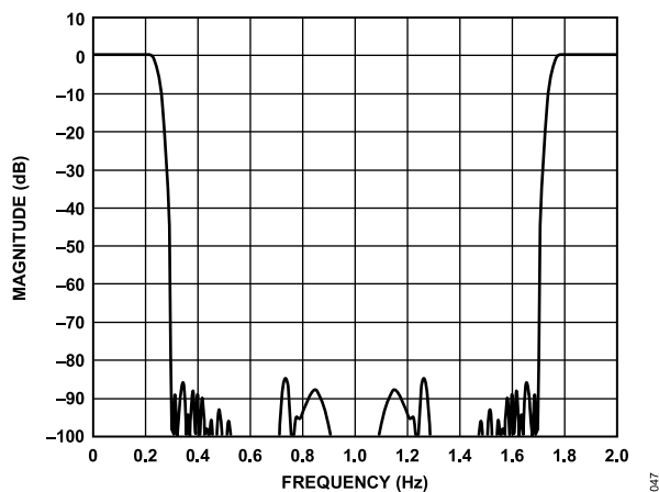
Figure 44. All-Band Response of 4x Mode
