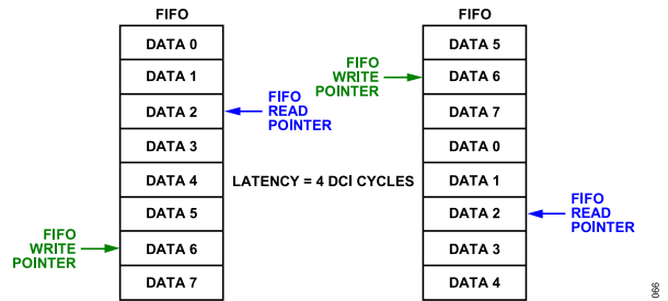
Figure 64. Example of Equal FIFO Latencies
