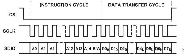
Figure 30. Serial Register Interface Timing, LSB First
