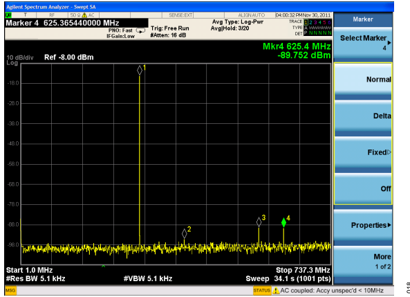
Figure 21. Single Tone f_{DAC} = 1474.56 MHz, f_{OUT} = 280 MHz, -14 dBFS
