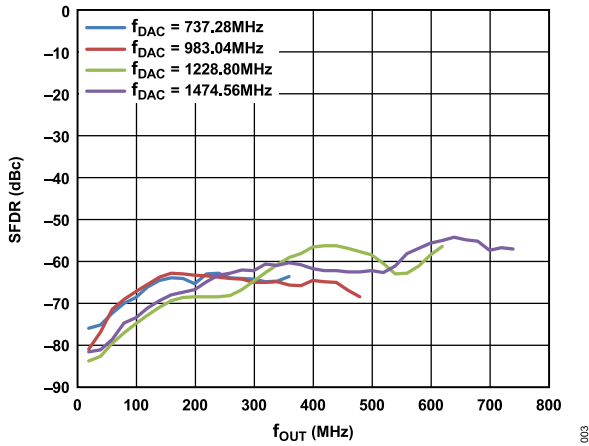
Figure 3. Single Tone (0 dBFS) SFDR vs. f_{OUT} in the First Nyquist Zone over Digital Back Off
