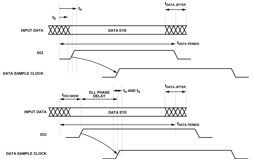
Figure 36. LVDS Data Port Timing Requirements
