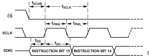
Figure 31. Timing Diagram for Serial Port Register Write
