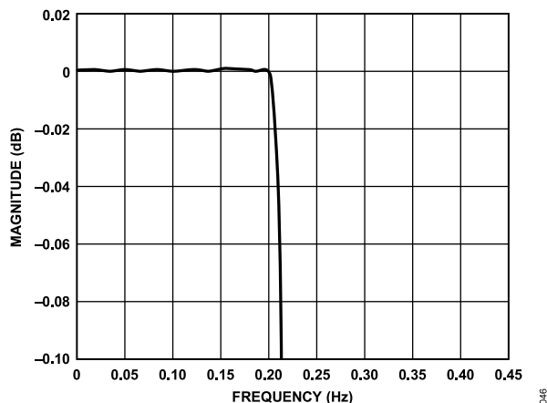
Figure 43. Pass-Band Detail of 4x Mode
