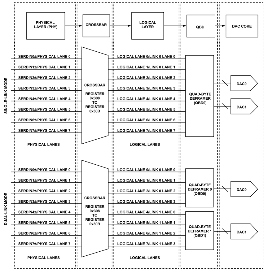
Figure 50. Link Mode Functional Diagram
