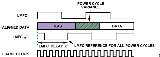
Figure 55. LMFC\_DELAY_x , to Compensate for Link Delay > LMFC
