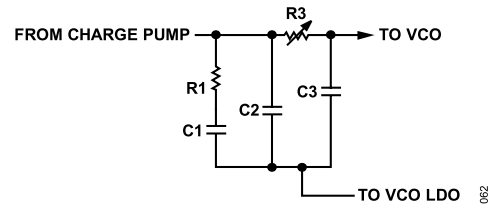
Figure 80. Loop Filter
