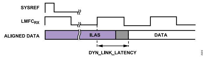
Figure 58. DYN_LINK_LATENCY Illustration
