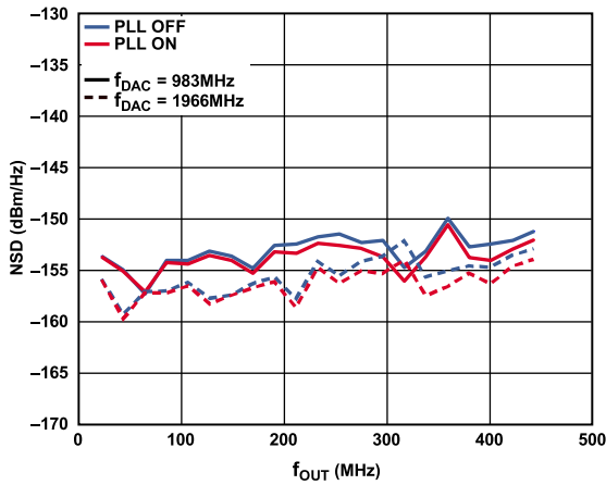
Figure 23. AD9135 Single-Tone NSD (0 dBFS) vs. f_{OUT} , f_{DAC} = 983 MHz and 1966 MHz, PLL On and Off
