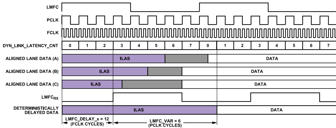
Figure 57. LMFC_DELAY_x Calculation Example
