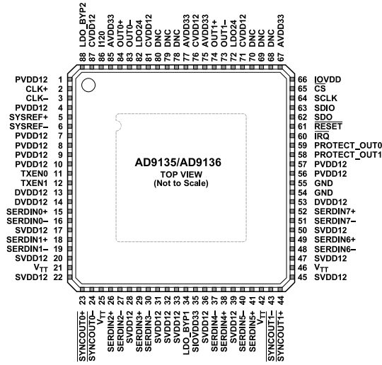
Figure 3. Pin Configuration
