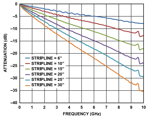
Figure 48. Insertion Loss of 50 Ω Striplines on FR4
