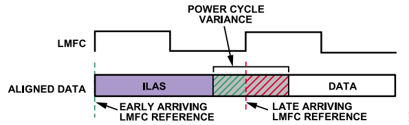
Figure 54. Link Delay > LMFC Period Example
