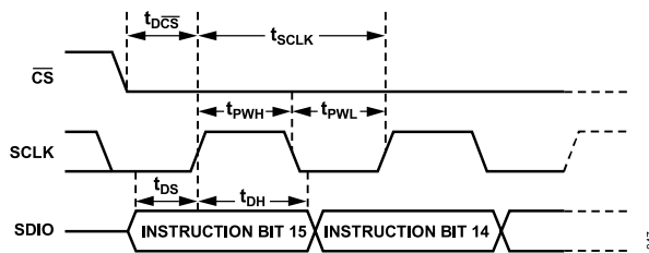
Figure 42. Timing Diagram for Serial Port Register Write
