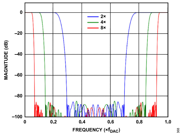
Figure 74. All Band Responses of Interpolation Filters
