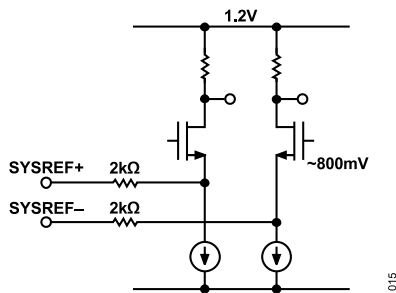
Figure 53. SYSREF \pm Input Circuit
