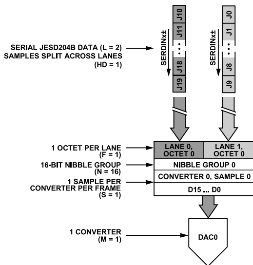
Figure 63. JESD204B Mode 9 Data Deframing
