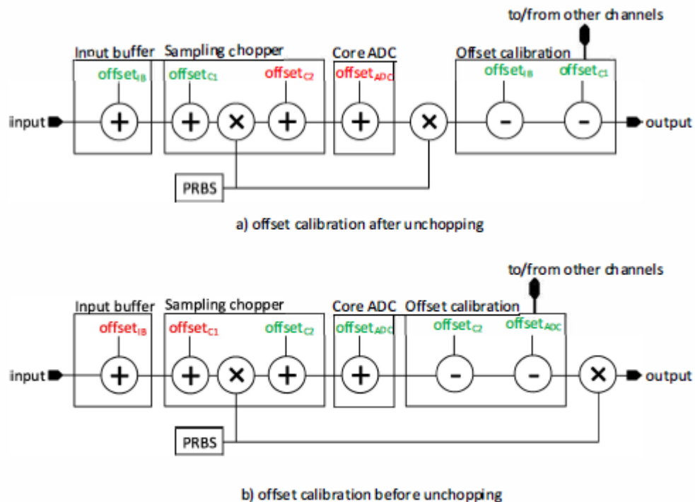
Fig.9. Offset sources in ADC and impact of where offset calibration is done.
