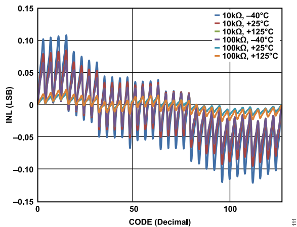
Figure 11. INL vs. Code (AD5123)
