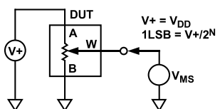
Figure 32. Potentiometer Divider Nonlinearity Error (INL, DNL)
