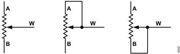
Figure 37. Rheostat Mode Configuration
