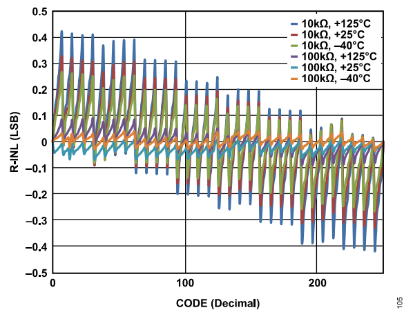
Figure 5. R-INL vs. Code (AD5143)
