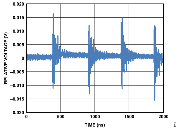
Figure 28. Digital Feedthrough
