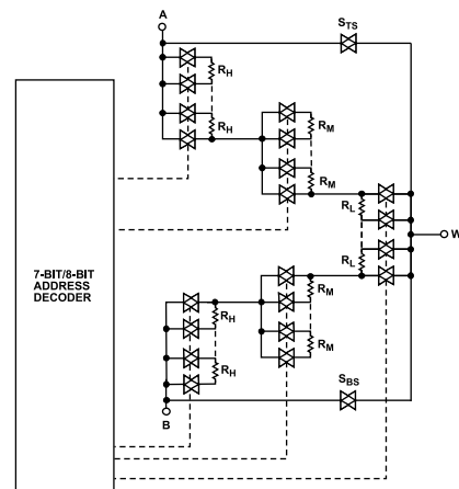
Figure 36. AD5123/AD5143 Simplified RDAC Circuit
