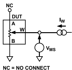
Figure 31. Resistor Integral Nonlinearity Error (Rheostat Operation; R-INL, R-DNL)
