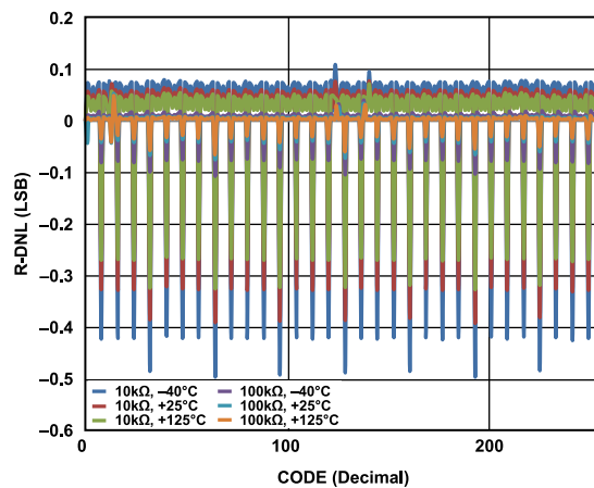
Figure 8. R-DNL vs. Code (AD5143)
