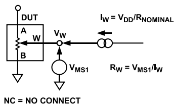
Figure 33. Wiper Resistance
