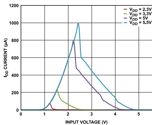
Figure 16. I_{DD} Current vs. Digital Input Voltage
