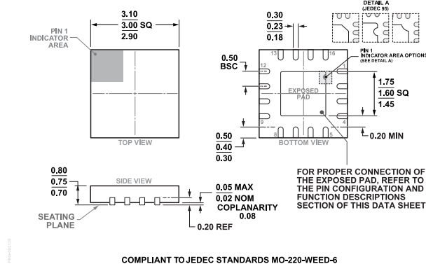
Figure 41. 16-Lead Lead Frame Chip Scale Package [LFCSP] 3 mm x 3 mm Body and 0.75 mm Package Height (CP-16-22) Dimensions shown in millimeter
