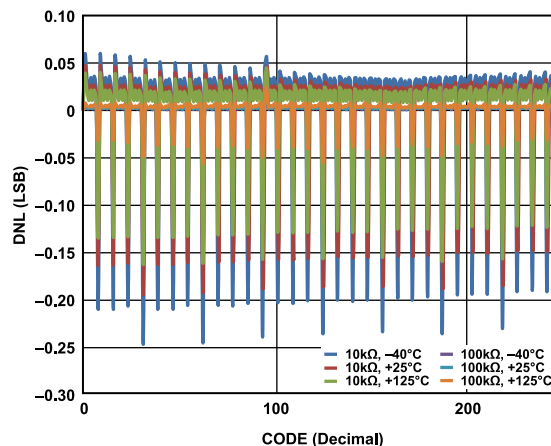
Figure 10. DNL vs. Code (AD5143)
