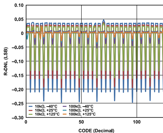
Figure 9. R-DNL vs. Code (AD5123)
