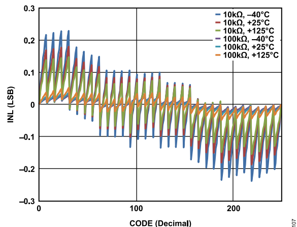
Figure 7. INL vs. Code (AD5143)
