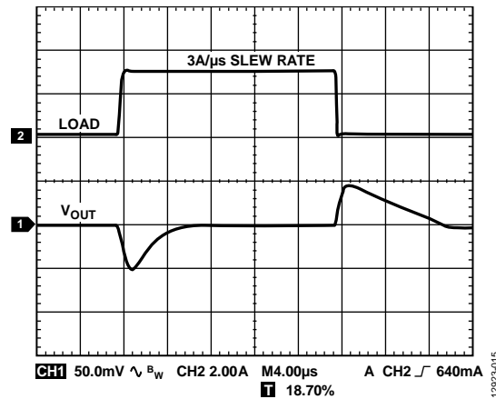
図 15. 負荷過渡応答、COUT = 47 μF、VIN = 1.8 V、VOUT = 1.3 V
