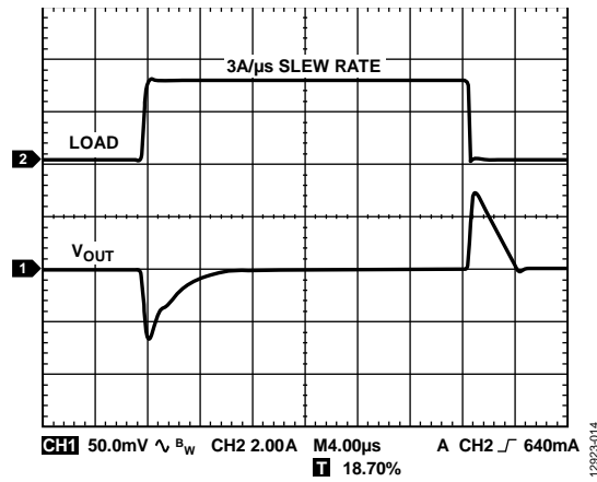
図 14. 負荷過渡応答、COUT = 10 μF、VIN = 1.8 V、VOUT = 1.3 V
