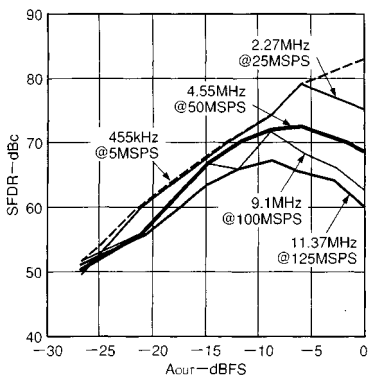
図27 . 1波のSFDRとA OUT @f OUT = f CLOCK /11
