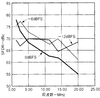
図6. SFDRとf OUT @50MSPS
