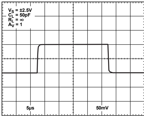
図26.小信号過渡応答
