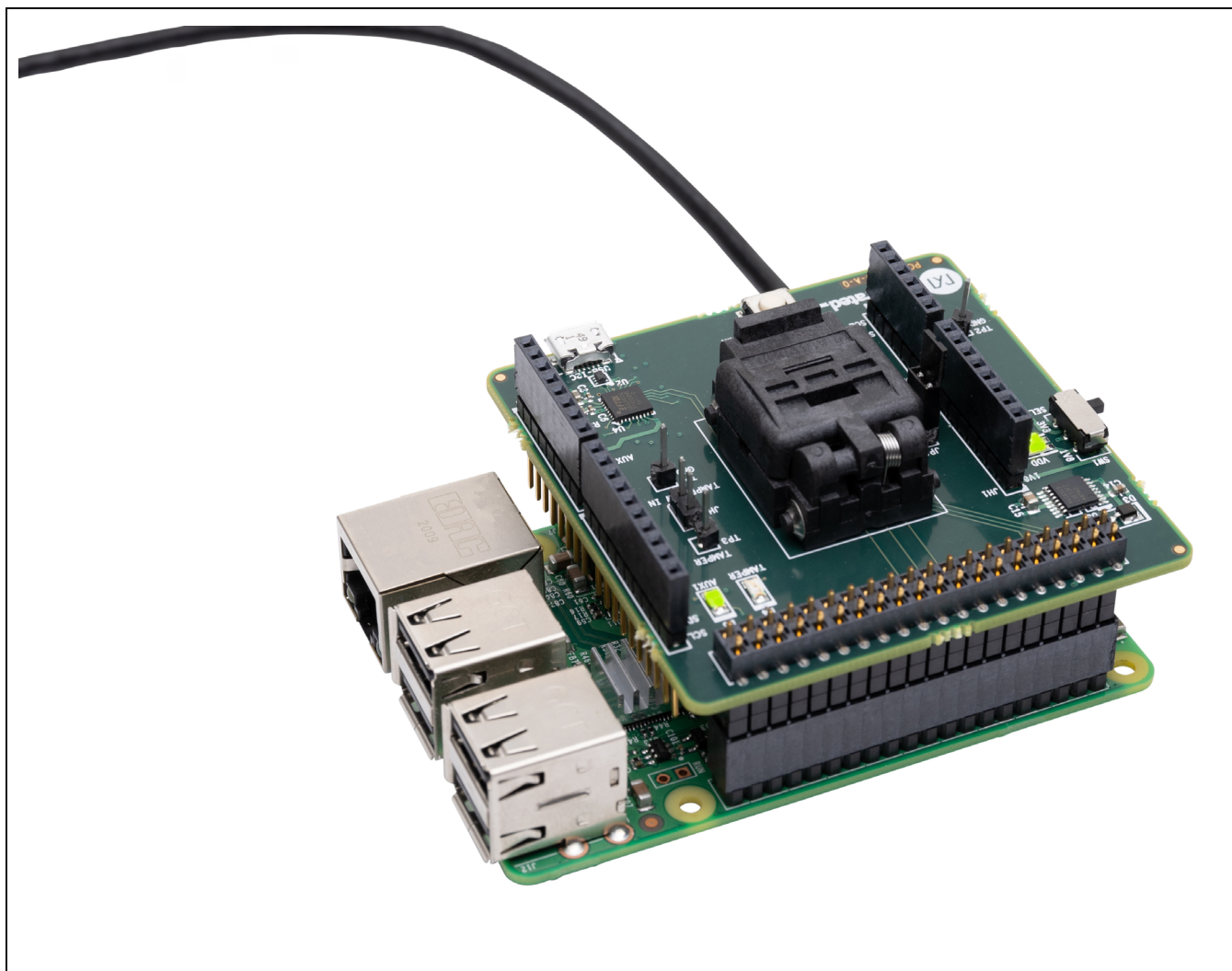
Figure 3. MAXQ1065 Socket Board Attached to Raspberry Pi through Elevated Header.
