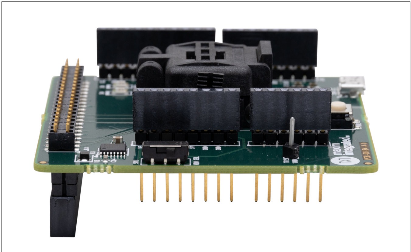
Figure 2. MAXQ1065 Socket Board with Elevated Header Installed.
