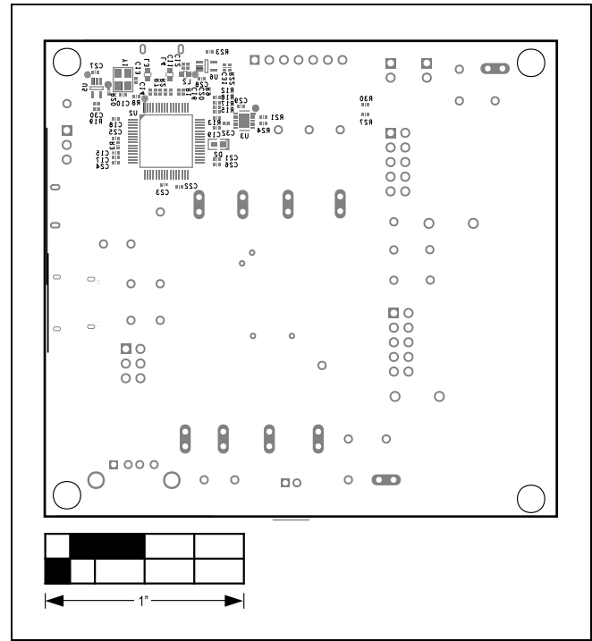
MAX77972 EV Kit Component Placement Guide—Bottom Silkscreen
