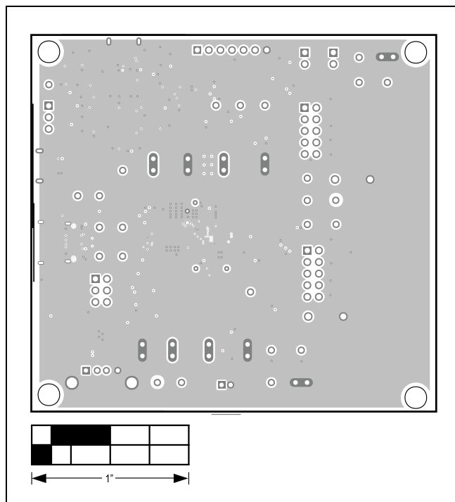
MAX77972 EV Kit PCB Layout—Layer 2
