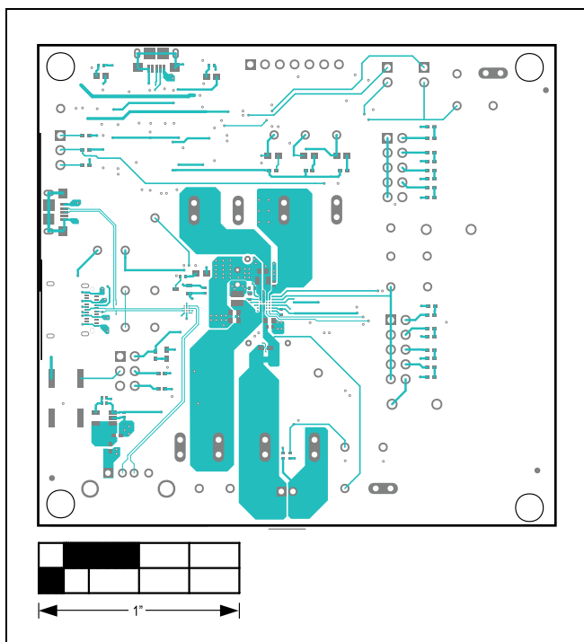
MAX77972 EV Kit PCB Layout—Top View
