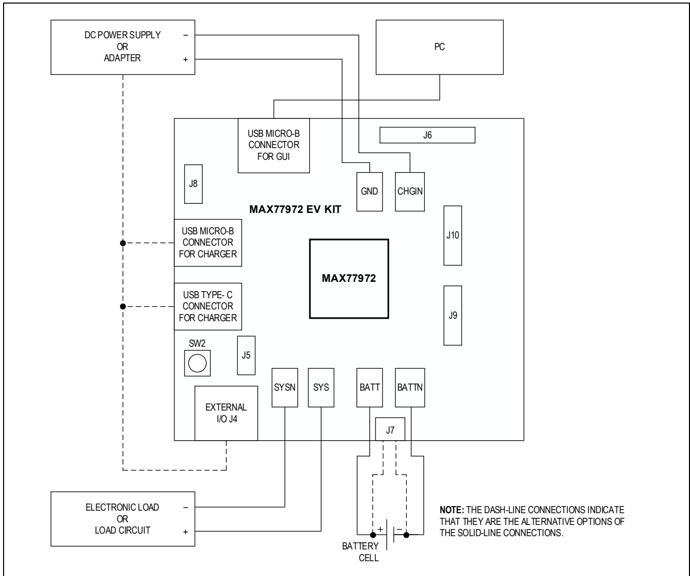
Figure 1. Board Connections
