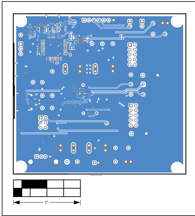
MAX77972 EV Kit PCB Layout—Bottom View
