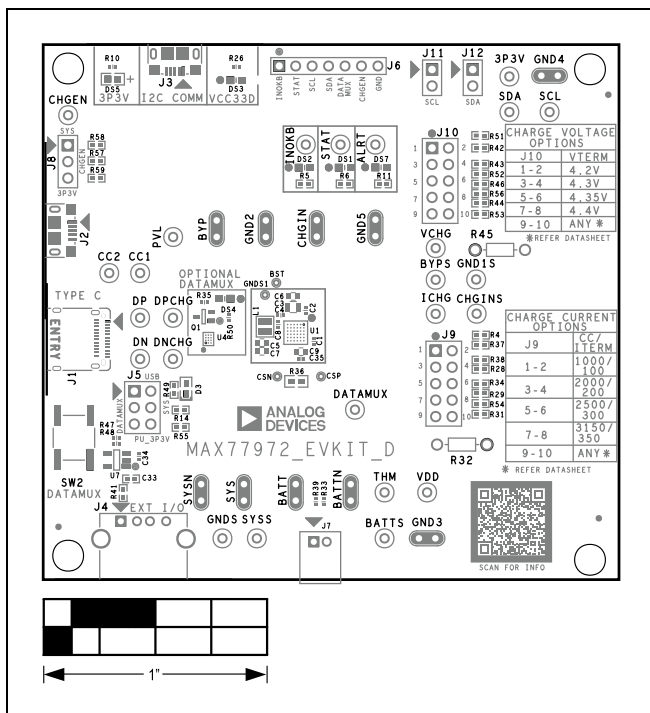
MAX77972 EV Kit Component Placement Guide—Top Silkscreen
