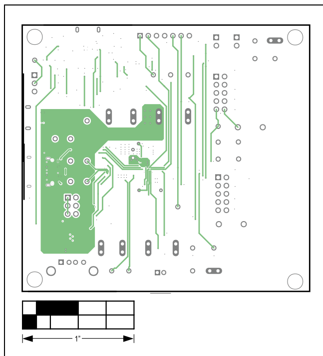
MAX77972 EV Kit PCB Layout—Layer 3
