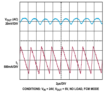
Figure 8. Steady-State Switching Waveform
