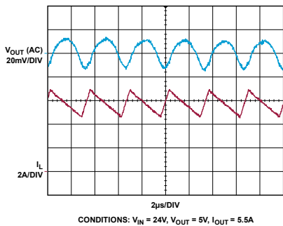
Figure 9. Steady-State Switching Waveform
