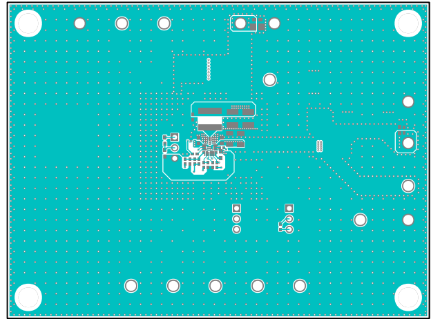
LT80605A EV Kit PCB Layout—Top
