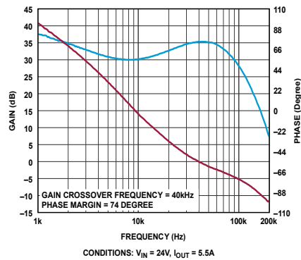
Figure 7. Gain/Phase vs Frequency
