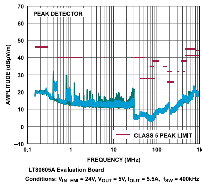
Figure 18. CISPR25 Radiated Emission Test with Class 5 Peak Limits
