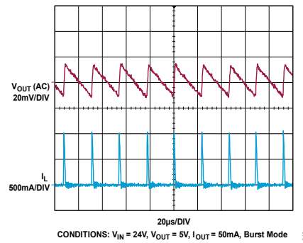
Figure 10. Steady-State Switching Waveform
