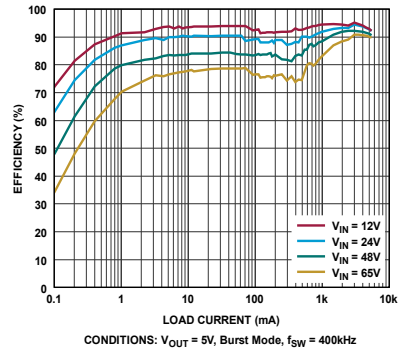
Figure 4. Efficiency vs Load Current
