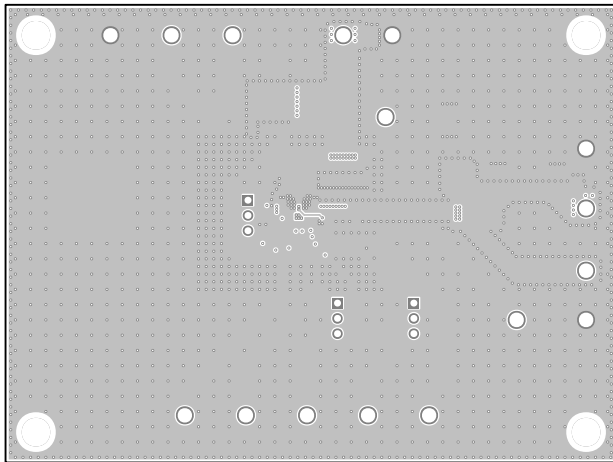
LT80605A EV Kit PCB Layout—Layer 2
