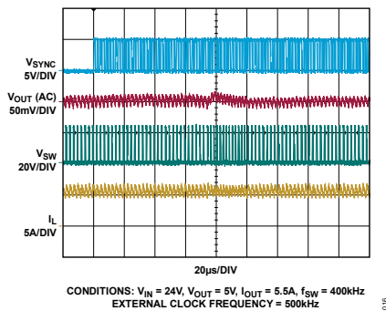
Figure 16. External Clock Synchronization
