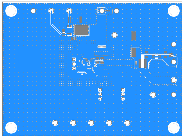
LT80605A EV Kit PCB Layout—Bottom
