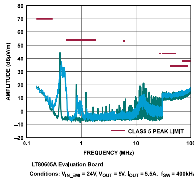
Figure 19. CISPR25 Conducted Emission Test with Class 5 Peak Limits
