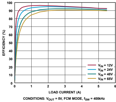
Figure 3. Efficiency vs Load Current
