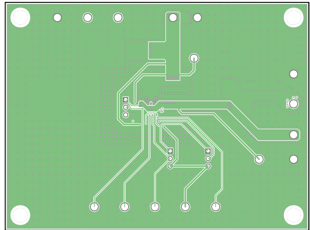
LT80605A EV Kit PCB Layout—Layer 3
