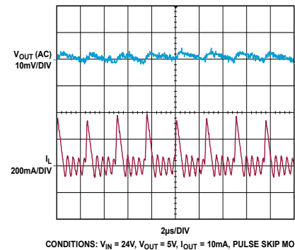
Figure 11. Steady-State Switching Waveform
