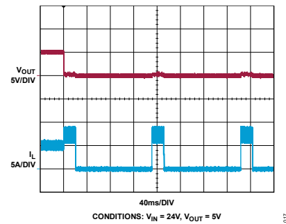
Figure 17. Output Short
