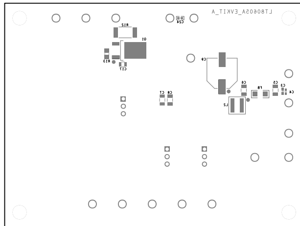
LT80605A EV Kit PCB Layout—Bottom Silkscreen
