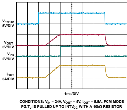
Figure 6. Startup/Shutdown through EN/UV
