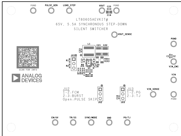
LT80605A EV Kit PCB Layout—Top Silkscreen
