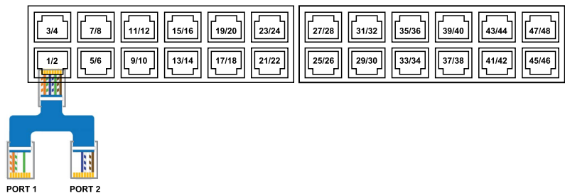
Figure 5. EVAL-LTC9101-2A/EVAL-LTC9101-2B Port Output Map
