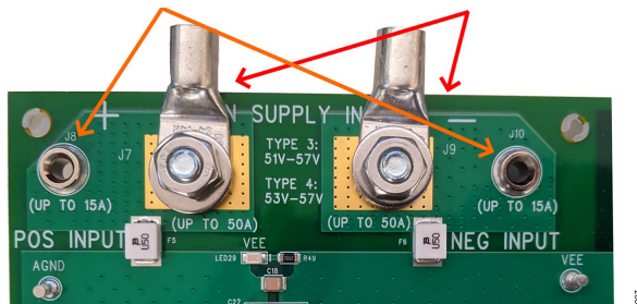
Figure 7. Motherboard Power Supply Connections
