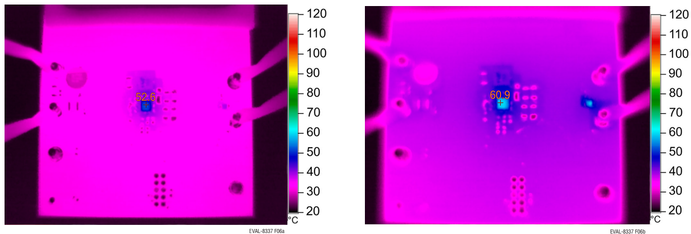
Figure 6. EVAL-LT8337-1-AZ Thermals
