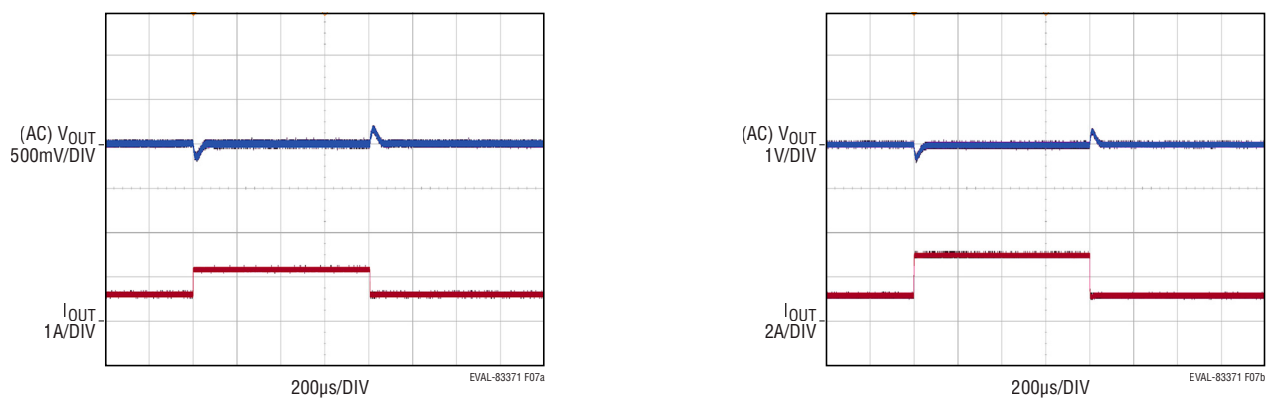
Figure 7. EVAL-LT8337-1-AZ V OUT Transient Response with JP1 = PULSE SKIP
