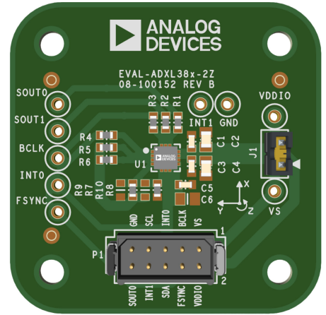
Figure 1. EVAL-ADXL382-2Z Evaluation Board Top View
