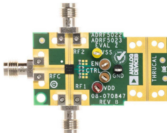
Figure 1. ADRF5031-EVALZ Evaluation Board Photograph
