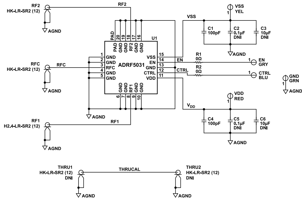
Figure 5. ADRF5031-EVALZ Evaluation Board Schematic
