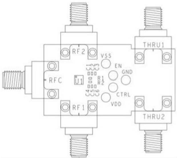
Figure 6. ADRF5031-EVALZ Evaluation Board Assembly Diagram
