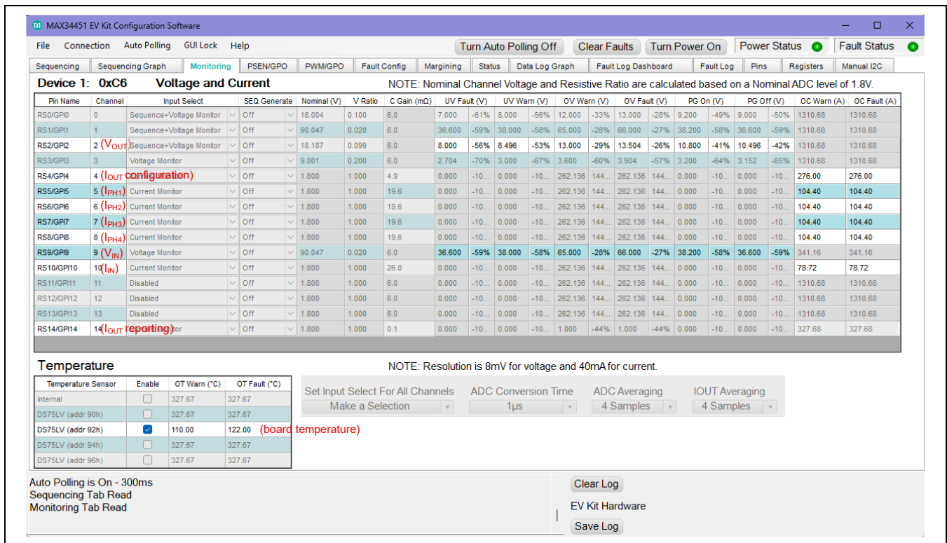
Figure 5. MAX34451 EV Kit GUI (Monitoring Tab)
