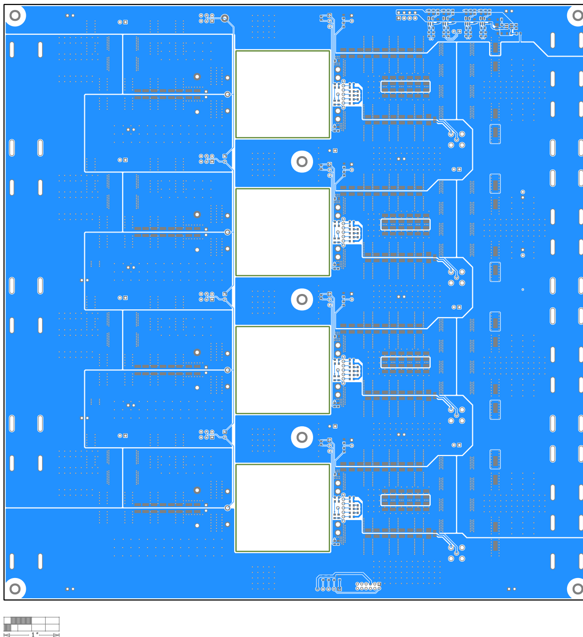
EVAL-ADPM12160 PCB Layout—Bottom
