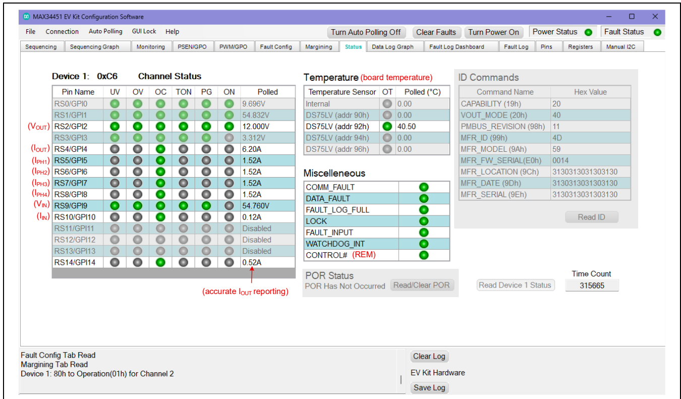
Figure 9. MAX34451 EV Kit GUI (Status Tab)
