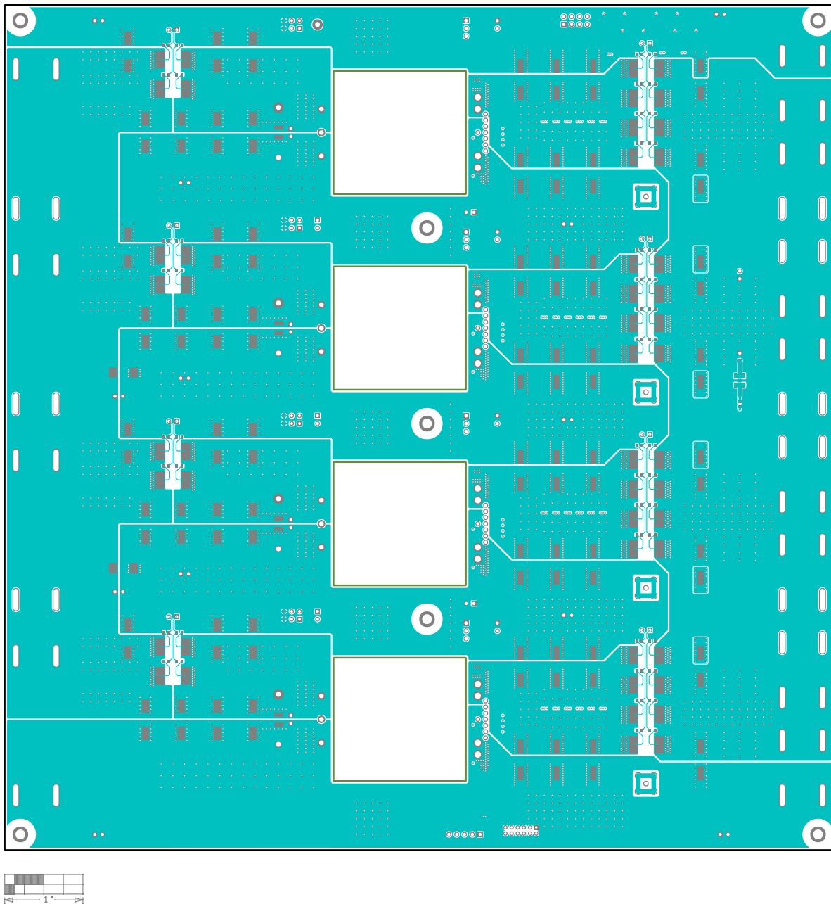
EVAL-ADPM12160 PCB Layout—Top
