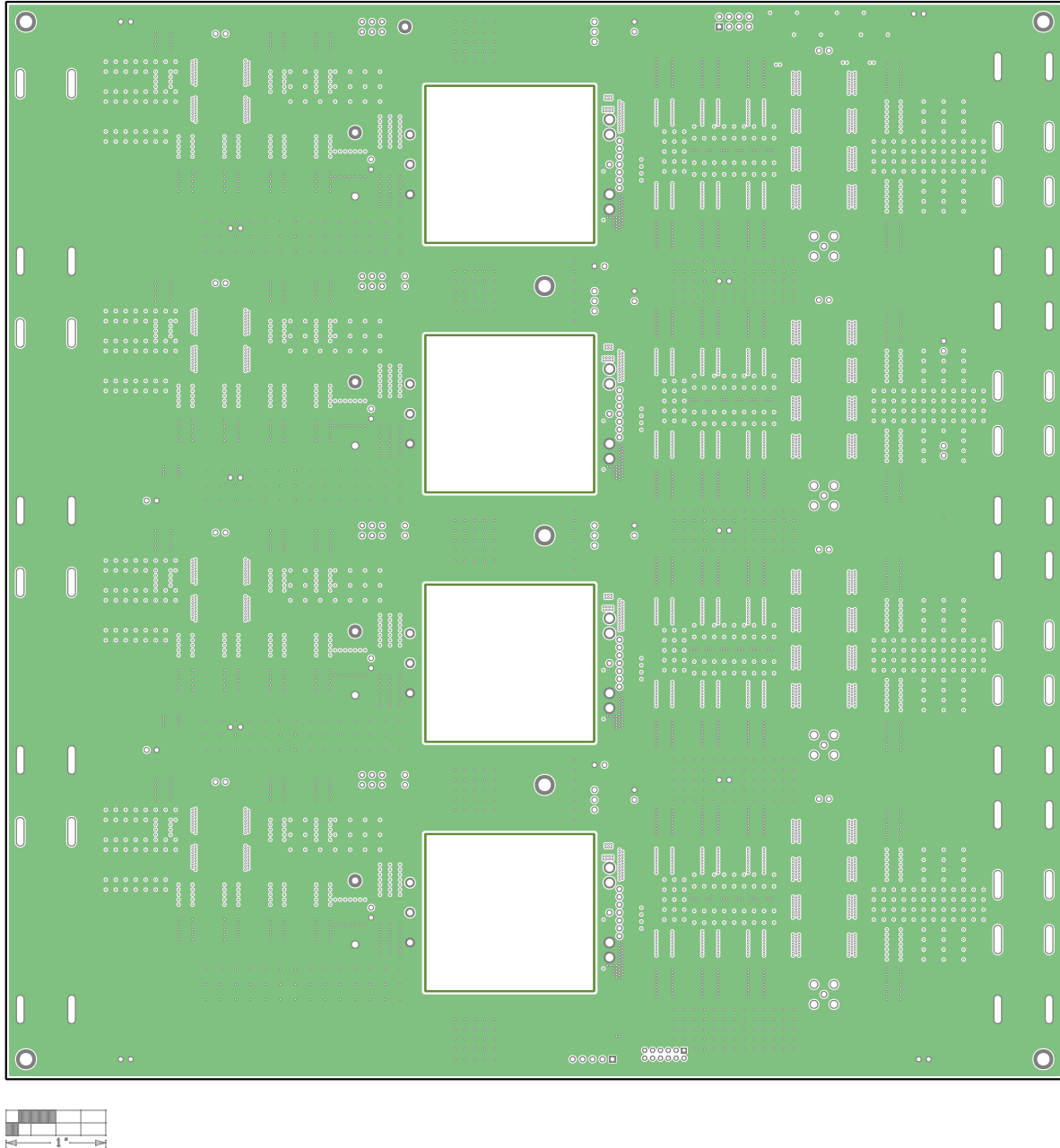
EVAL-ADPM12160 PCB Layout—Layer 3
