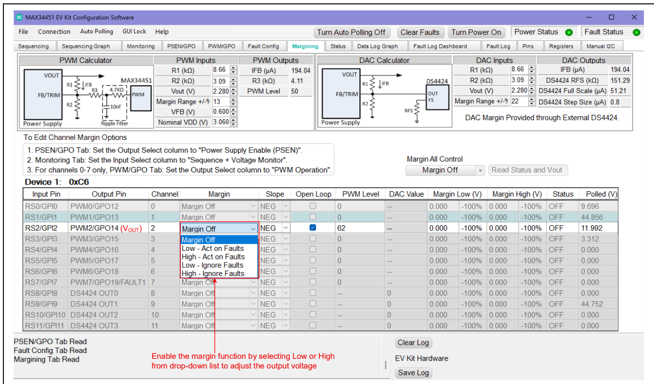
Figure 8. MAX34451 EV Kit GUI (Margining Tab)
