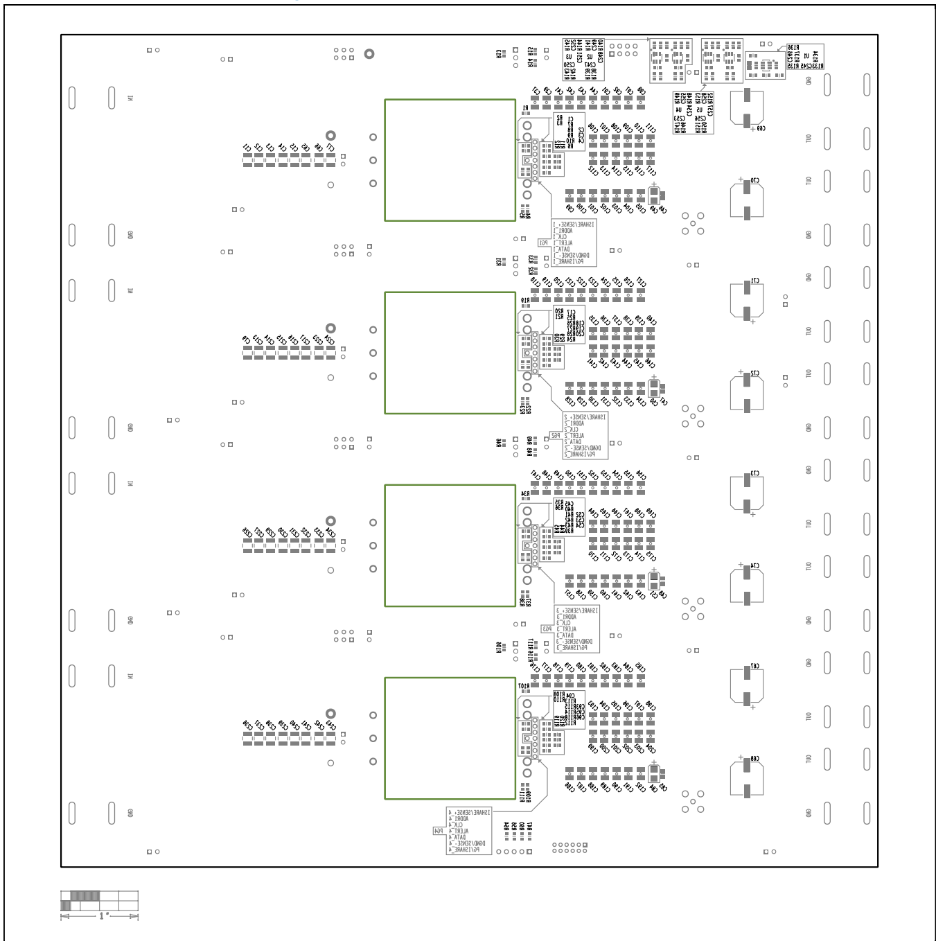
EVAL-ADPM12160 Component Placement—Bottom Silkscreen
