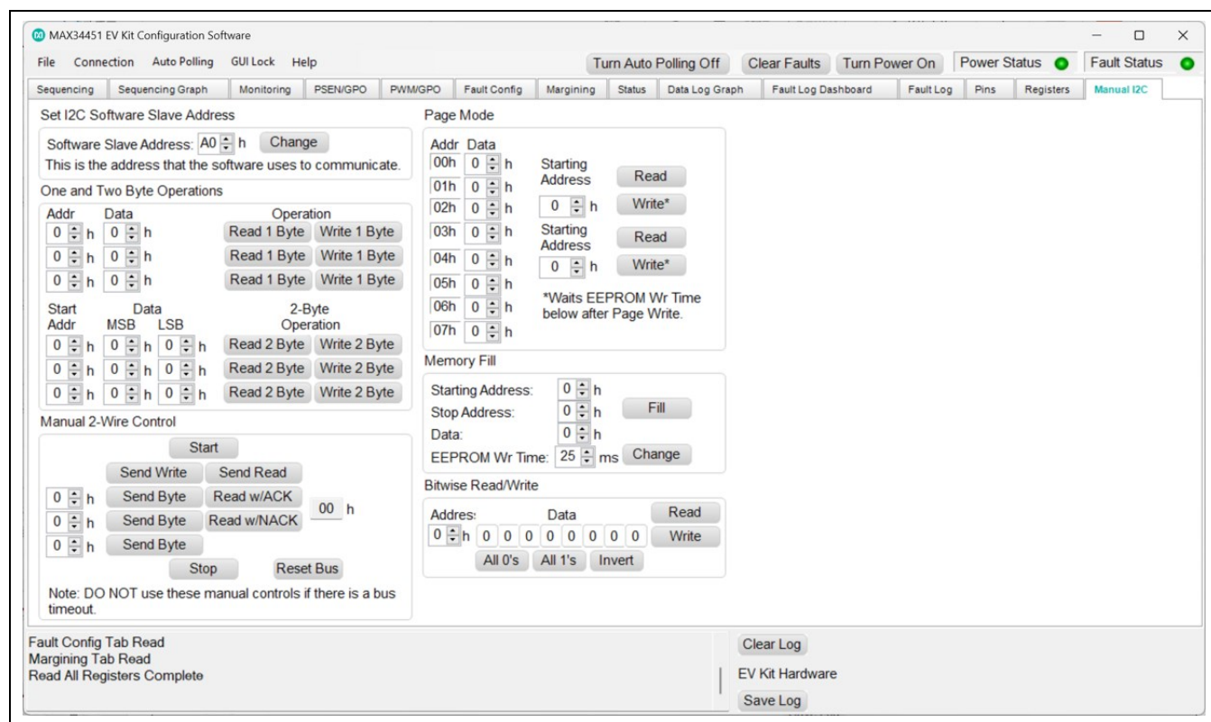
Figure 14. MAX34451 EV Kit GUI (Manual I 2 C Tab)
