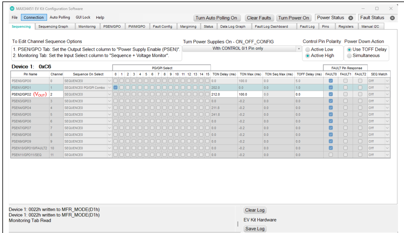
Figure 3. MAX34451 EV Kit GUI (Sequencing Tab)
