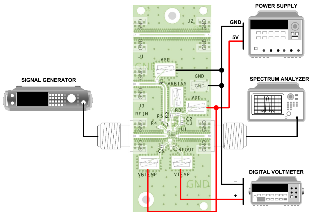
Figure 3. ADL8108-EVALZ Operating Block Diagram
