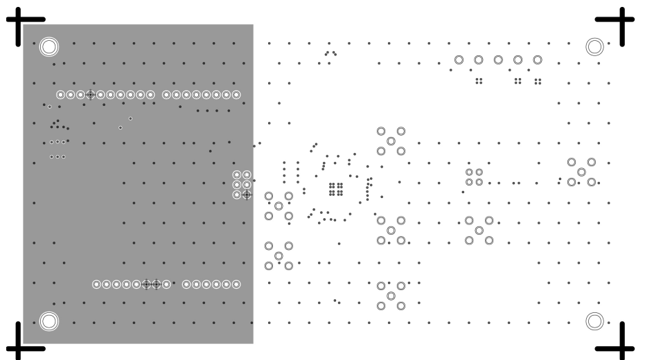
Figure 9. AD9951/PCBZ-SDP-K1 Schematic, Ground
