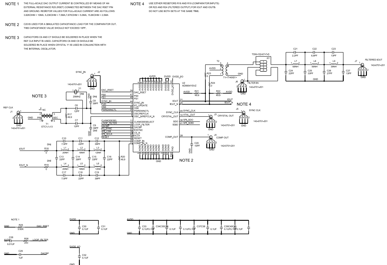
Figure 7. AD9859/PCBZ-SDP-K1 Schematic, Page 3
