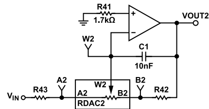
Figure 14. Linear Inverting Amplifier
