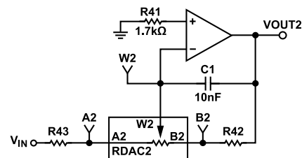
Figure 15. Pseudologarithmic Inverting Amplifier
