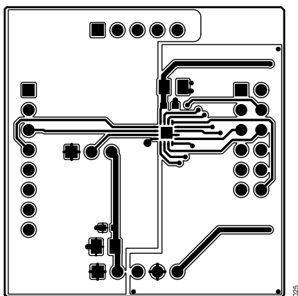
Figure 24. Component Side View of EVAL-AD5143-2DBZ
