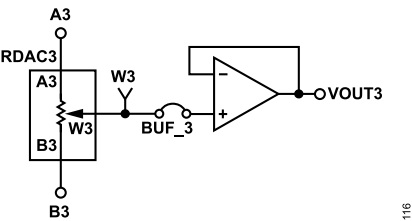
Figure 16. RDAC3
