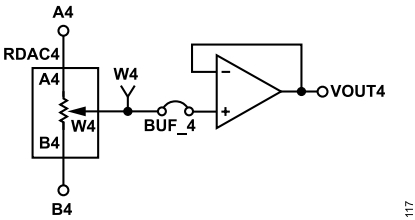
Figure 17. RDAC4
