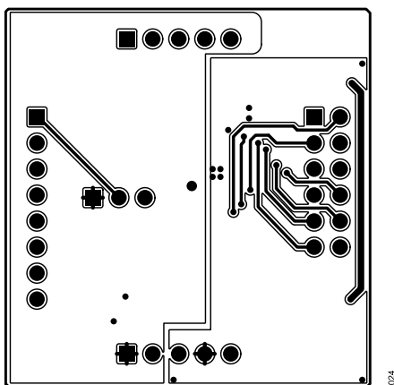
Figure 25. Component Placement Drawing of EVAL-AD5143-2DBZ
