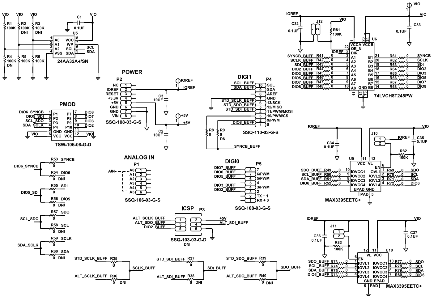
Figure 18. EVAL-MB-LV-ARDZ Schematic, SDP, Arduino-Compatible, PMOD Connectors, and Translators
