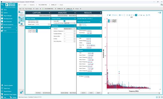
Figure 18. Increasing SNR with the Integrated Digital Filter
