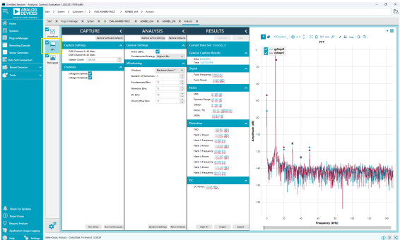
Figure 15. Data Set Plotted in the Frequency Domain
