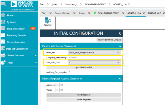
Figure 17. Digital Filter Configuration from the AD4883 Tab in the ACE Software
