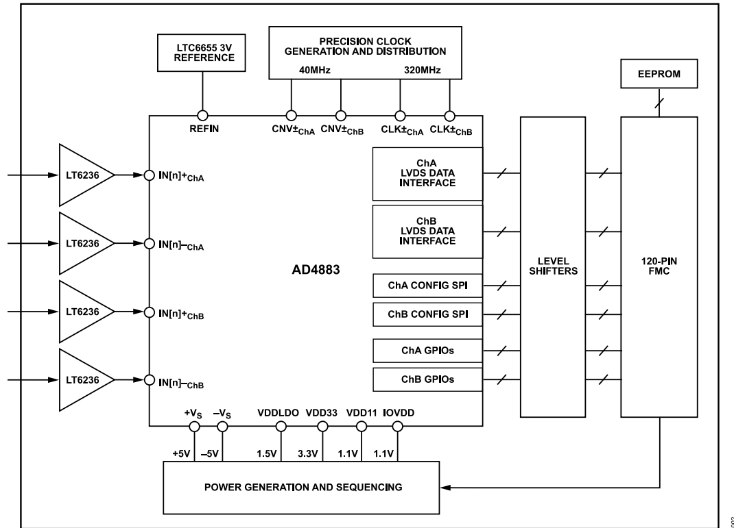
Figure 2. Simplified Block Diagram of the EVAL-AD4883-FMCZ
