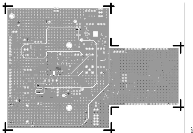
Figure 37. EVAL-AD4190-4ARDZ Layer 3 Power
