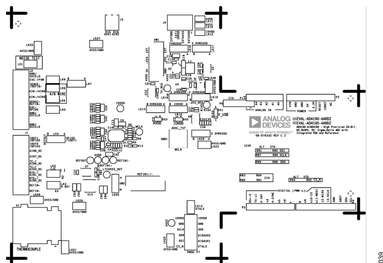
Figure 39. EVAL-AD4190-4ARDZ Silkscreen Primary
