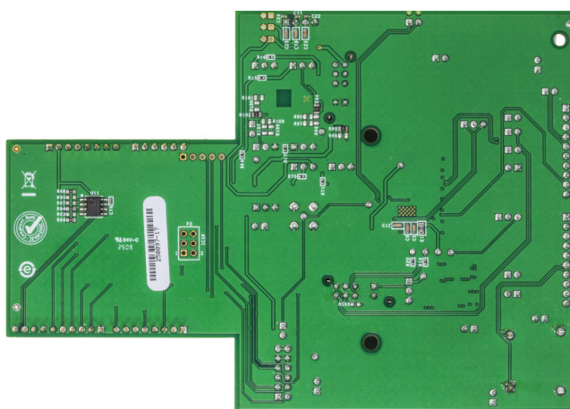
Figure 2. EVAL-AD4190-4ARDZ Evaluation Board Photograph — Bottom
