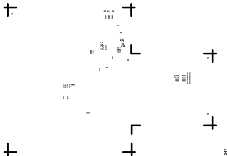
Figure 44. EVAL-AD4190-4ARDZ Pastemask Secondary
