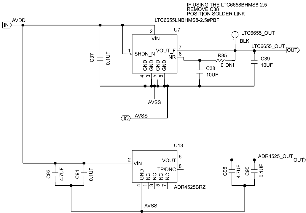
Figure 33. EVAL-AD4190-4ARDZ Schematic Part 5
