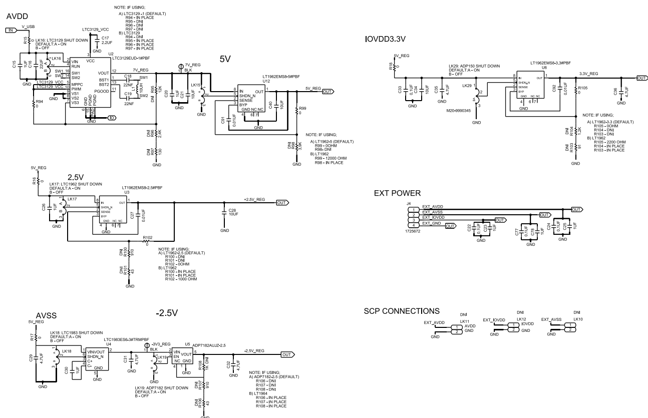
Figure 30. EVAL-AD4190-4ARDZ Schematic Part 2
