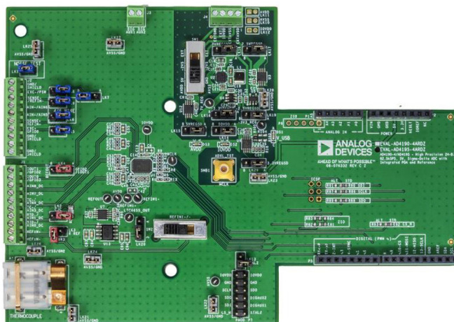
Figure 1. EVAL-AD4190-4ARDZ Evaluation Board Photograph — Top
