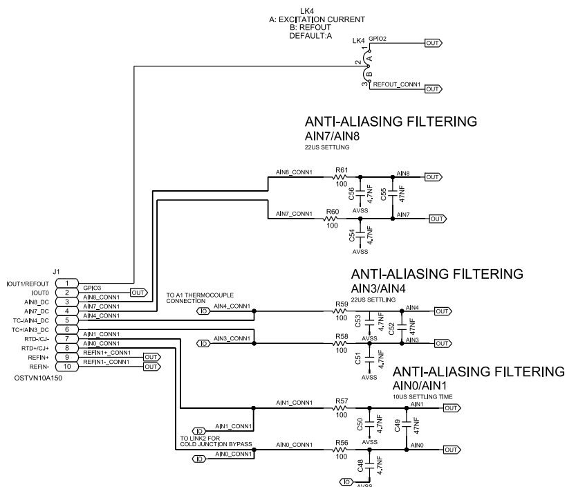
Figure 34. EVAL-AD4190-4ARDZ Schematic Part 6
