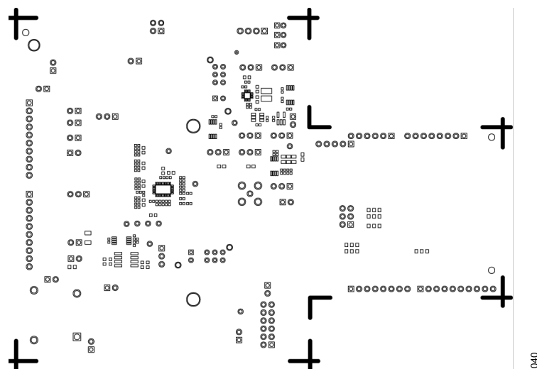
Figure 40. EVAL-AD4190-4ARDZ Soldermask Primary
