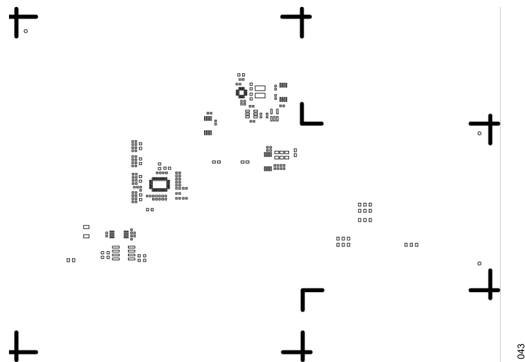
Figure 43. EVAL-AD4190-4ARDZ Pastemask Primary
