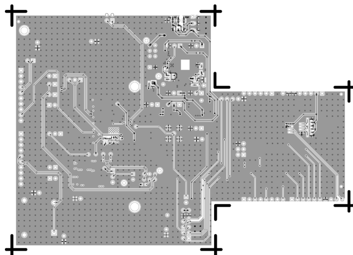
Figure 38. EVAL-AD4190-4ARDZ Layer 4 Secondary
