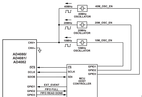
Figure 9. Simplified Diagram of the Clock Circuitry
