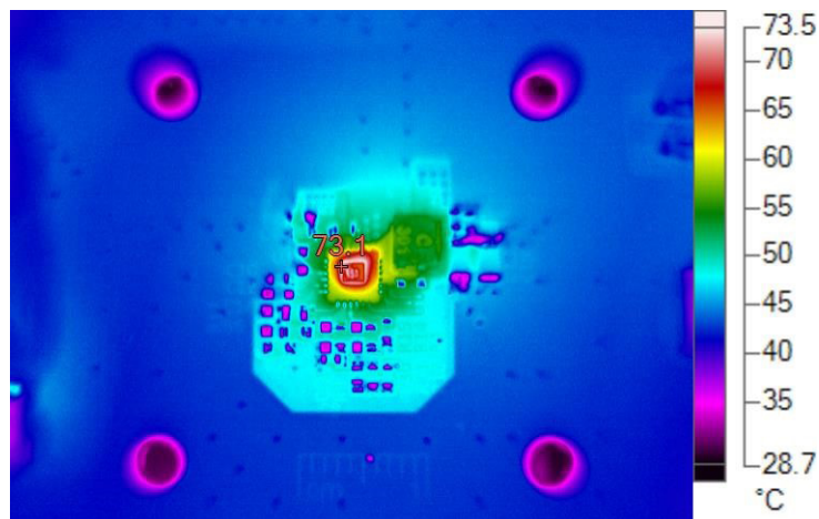
Figure 7. Thermal Performance at V IN = 12V, f SW = 2MHz, V OUT = 1V, I LOAD = 8A, T A = 25°C
