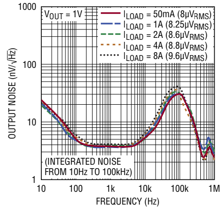
Figure 4. LT8625SP-1 Demo Circuit DC3220A Noise Spectral Density (12V Input to 1V Output, f_{SW} = 2\text{MHz} )
