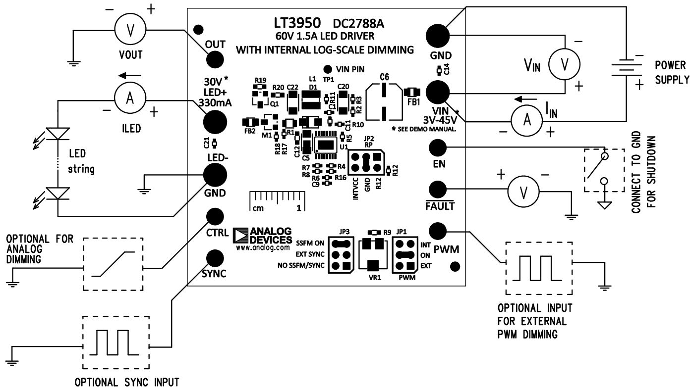
Figure 1. Test Procedure Setup Drawing for DC2788A
