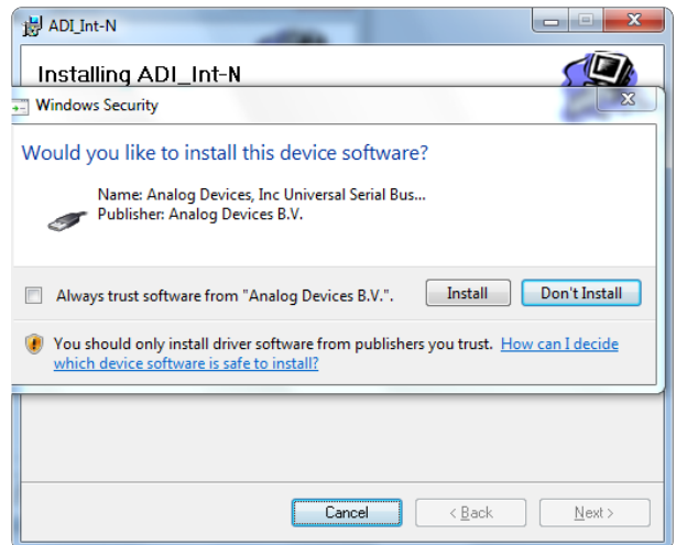
Figure 16. Software Installation
