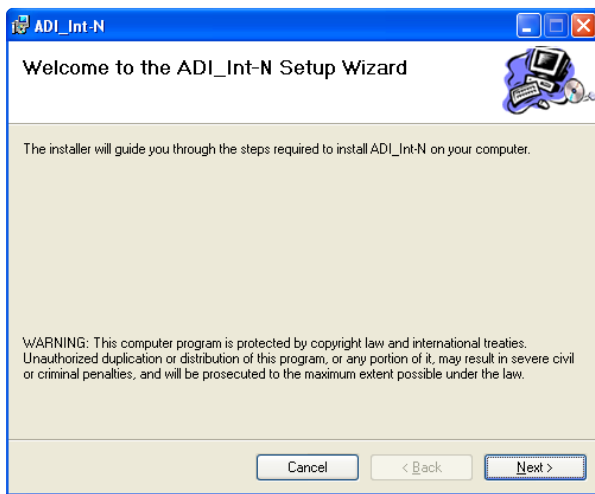
Figure 1. Setup Wizard
