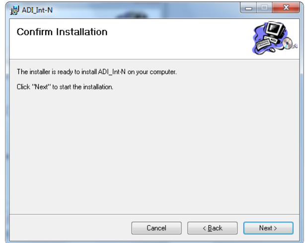
Figure 15. Confirm Installation
