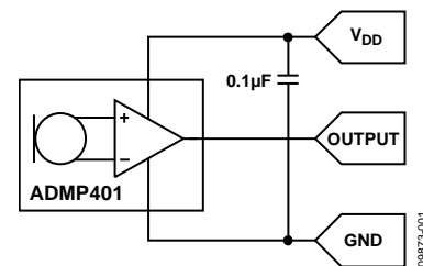
Figure 1. Evaluation Board Schematic
