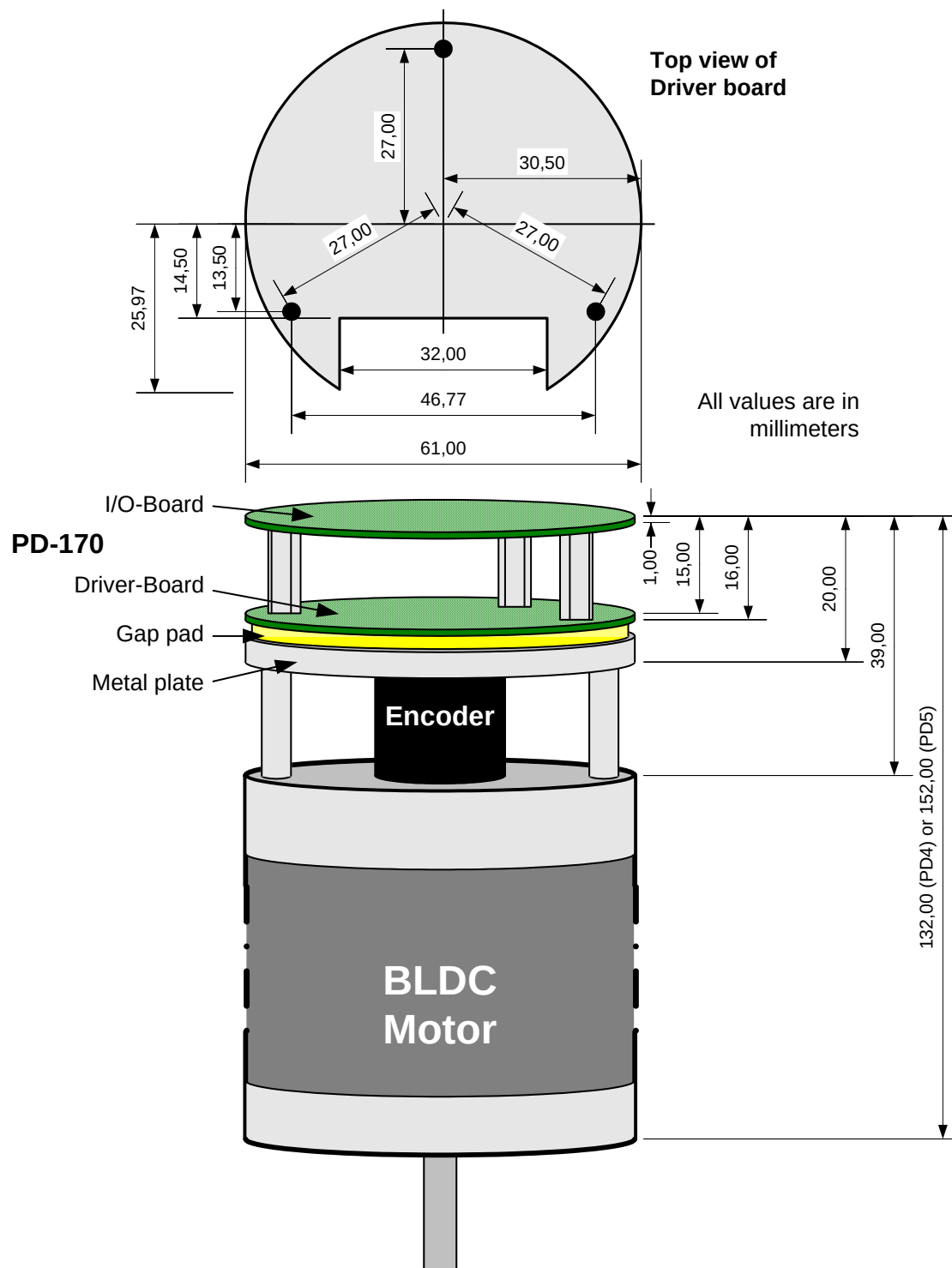
Figure 4.3: Dimensions of TCM-170 and PD-170
