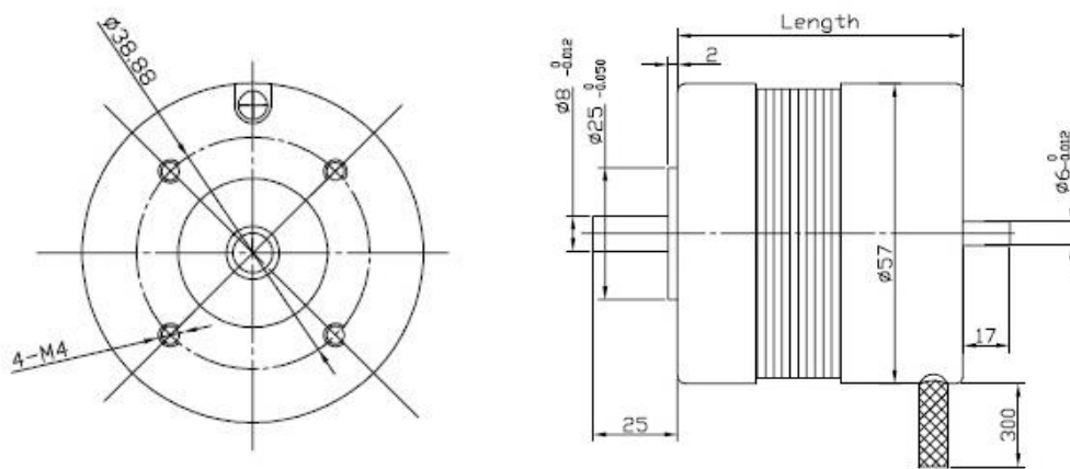
Figure 4.4: Motor dimensions
