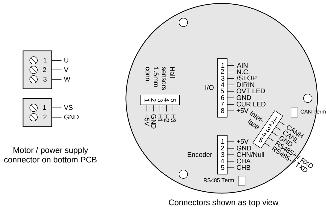
Figure 4.1: Pinning
