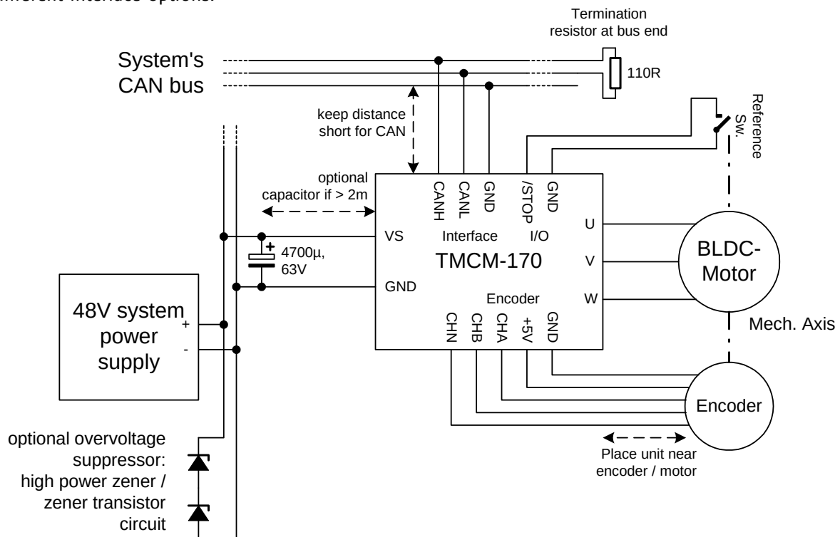
Figure 4.2: Application circuit
