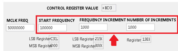
Figure 3. Frequency Output
