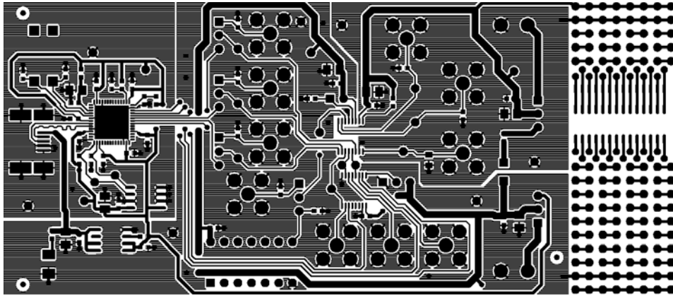
Figure 10. EVAL-AD5932EBZ Component Side Artwork
