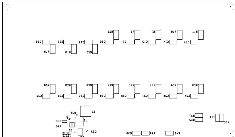
Figure 12. EVAL-AD5679RSDZ Bottom Side Component Placement
