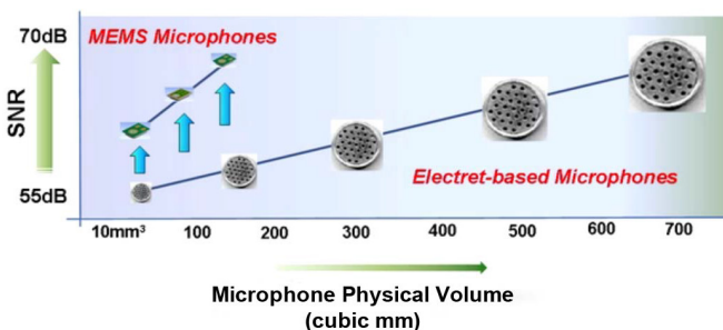
MEMS Microphones vs. ECMs MEMS Mics Offer Greater Performance Density
