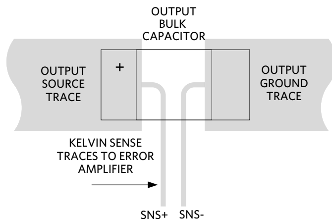
Figure 29. Proper Kelvin Sense Connections
