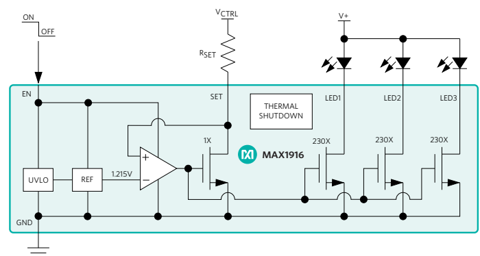
Figure 42. MAX1916 Linear LED Driver
