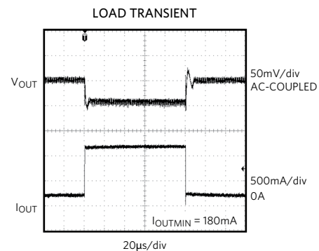
Figure 31. Load Step with Voltage Positioning
