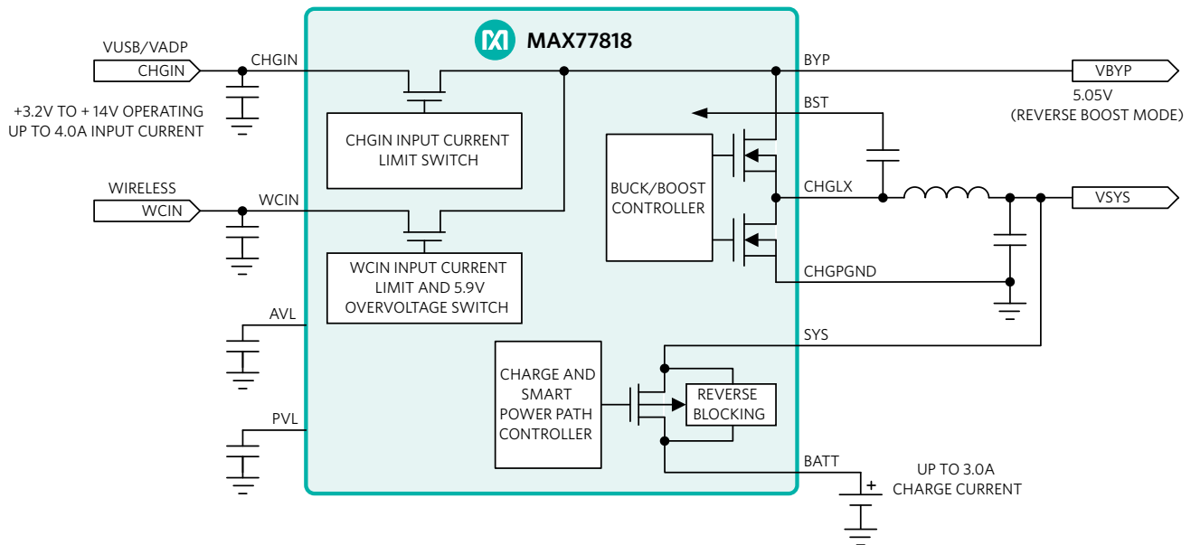
Figure 16. MAX77818 Typical Operating Circuit
