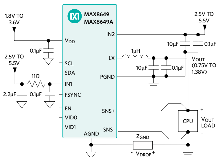
Figure 28. MAX8649/MAX8649A with Differential Feedback to Bypass GND Impedance
