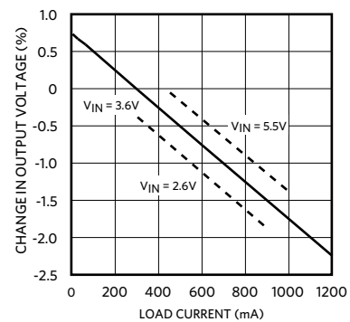
Figure 33. MAX1556 Voltage Positioning Load Line
