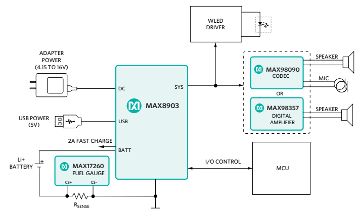
Figure 15. Digital Camera Application Using the MAX8903 Switch-Mode Charger
