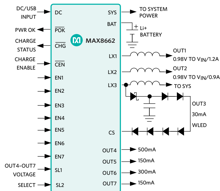
Figure 5. MAX8662 Typical Operating Circuit
