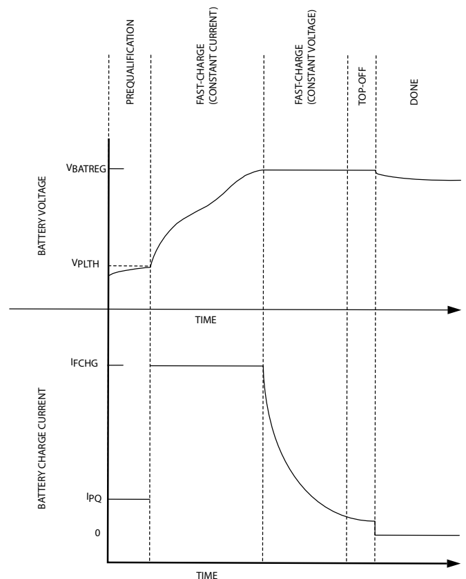
Figure 12. Charging Stages for Safe Charging
