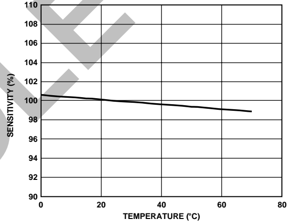
Figure 7. Normalized Sensitivity vs. Temperature
