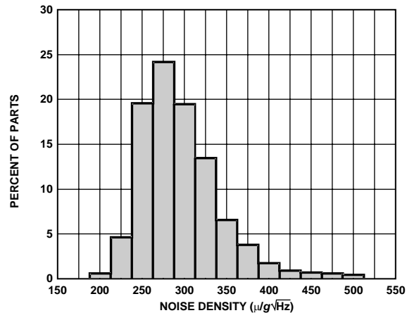
Figure 8. Noise Density Distribution
