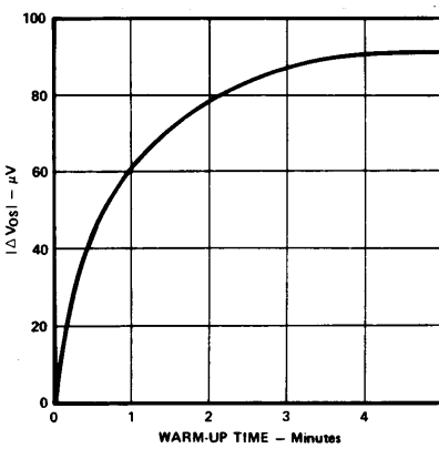
Figure 8. Change in Offset vs. Warm-Up Time
