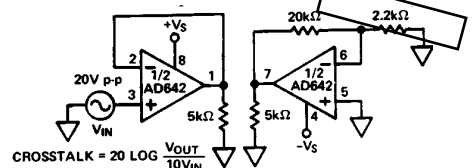
Figure 20. Crosstalk Test Circuit
