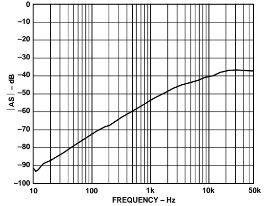
Figure 10. Audio Susceptibility (Magnitude of V_{OUT}/V_{IN} )
