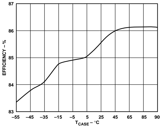
Figure 3. Efficiency vs. Case Temperature (°C) (at Nominal V_{IN} , 75% Max Load, ADDC02812DA)
