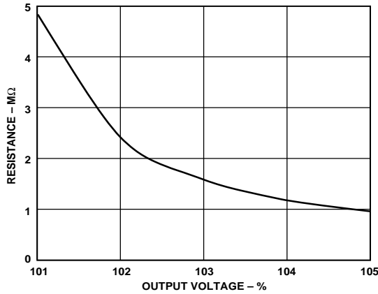
Figure 19. External Resistor Value for Increasing Output Voltage
