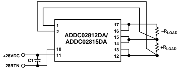
Figure 28. Typical Power Connections and External Parts for Converter
