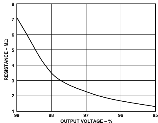
Figure 18. External Resistor Value for Reducing Output Voltage
