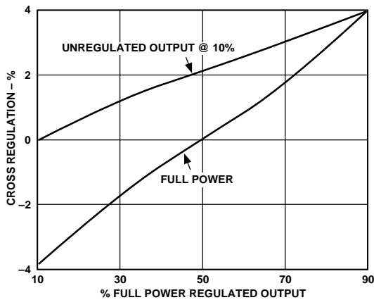
Figure 9. Cross Regulation Envelope
