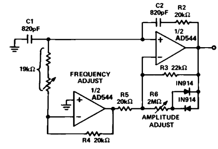
Figure 36. Wien-Bridge Oscillator- f_0 = 10 kHz
