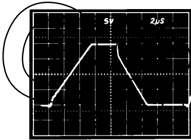
Figure 21a. Unity Gain Follower Pulse Response (Large Signal)
