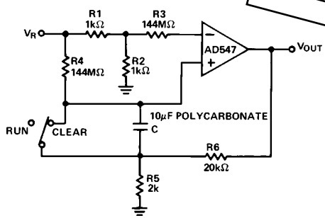
Figure 38. Long Interval Timer-1,000 Seconds
