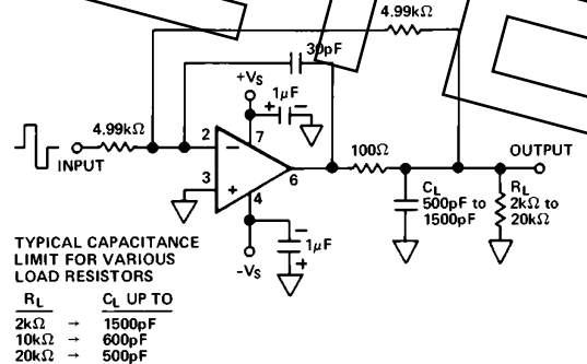
Figure 27. Circuit for Driving a Large Capacitance Load
