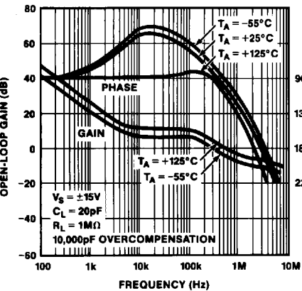
OPEN-LOOP GAIN, PHASE vs FREQUENCY ( C_{OC} = 10,000pF )
