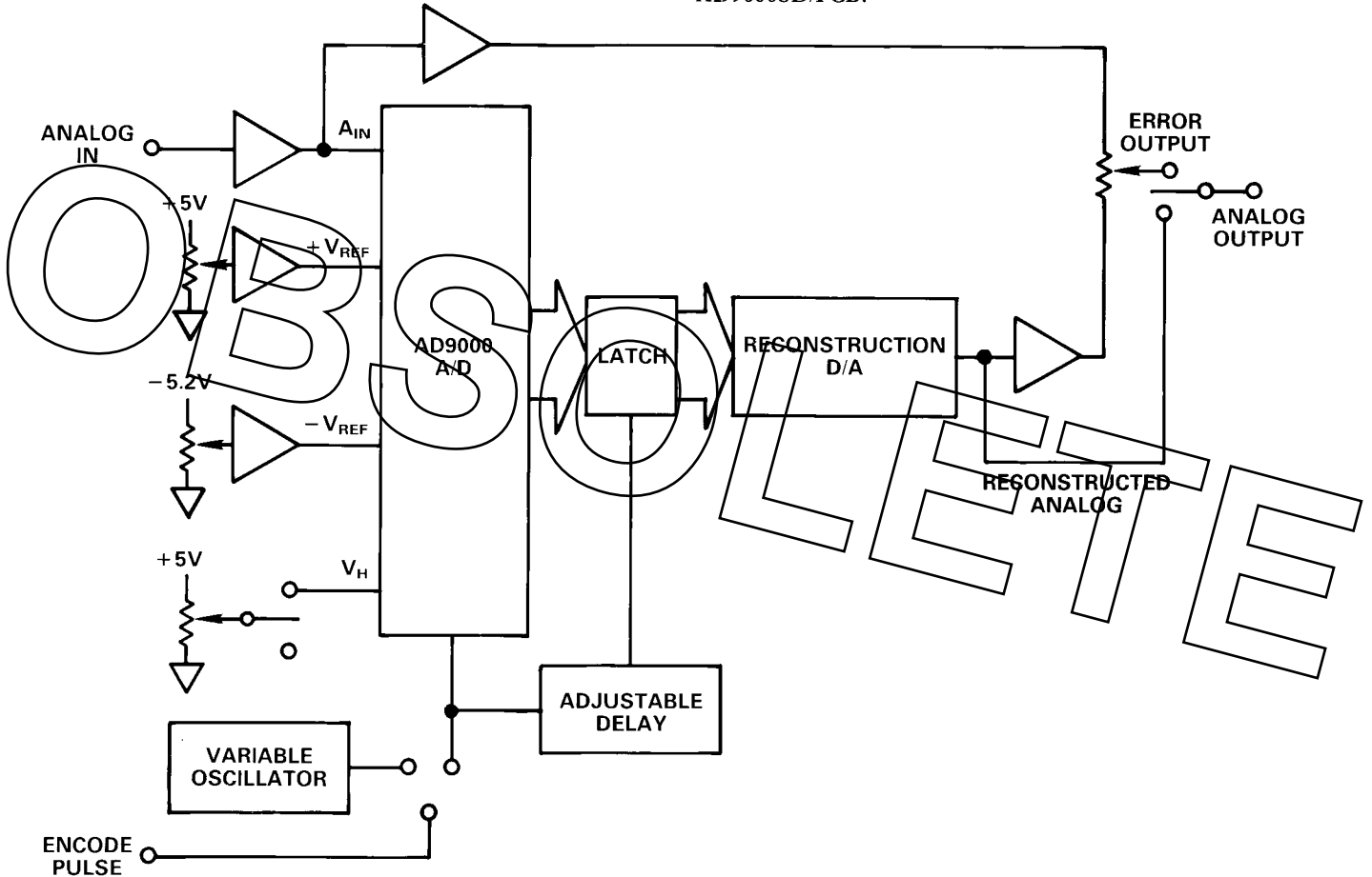
AD9000/PCB Block Diagram
