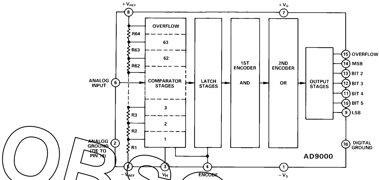
AD9000 Functional Block Diagram
