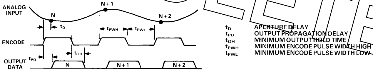
System Timing Diagram
