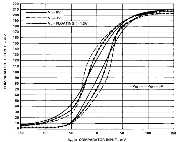
Comparator Switching vs. Hysteresis Voltage
